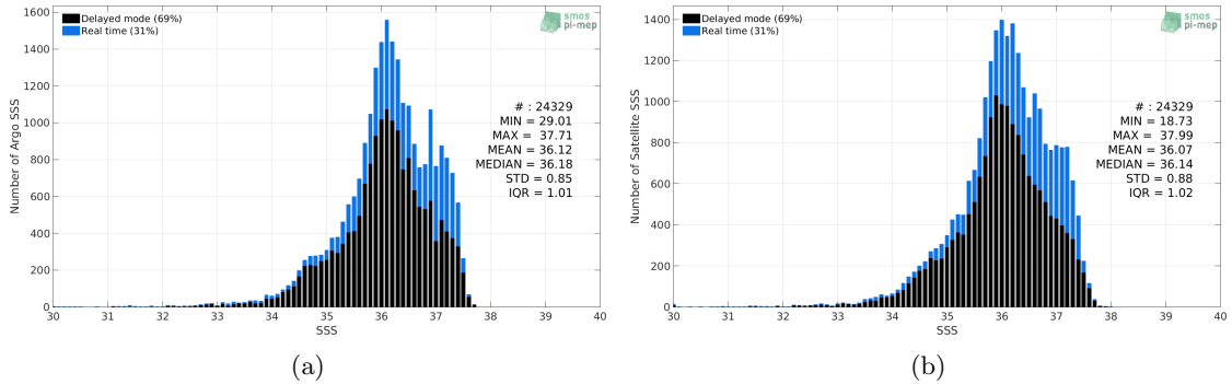
Figure 2: Histograms of SSS from Argos (a) and Aquarius-L3-OR-V5-7DAY-RUNNING-1DEG (b) considering all match-up pairs per bins of 0.1 over the Tropical Atlantic Ocean Pi-MEP region and for the full satellite product period.
