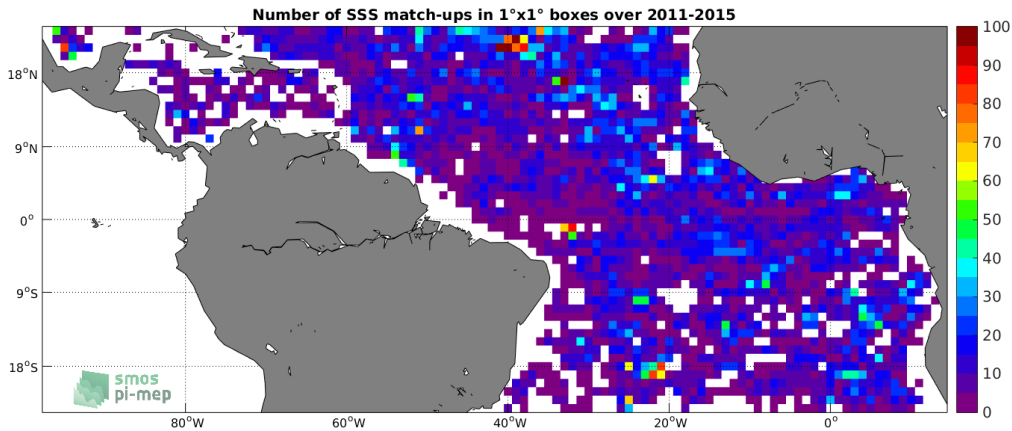
Figure 4: Number of SSS match-ups between Argo SSS and the Aquarius-L3-OR-V5-7DAY-RUNNING-1DEG SSS product for the Tropical Atlantic Ocean Pi-MEP region over 1^\circ \times 1^\circ boxes and for the full satellite product period.
