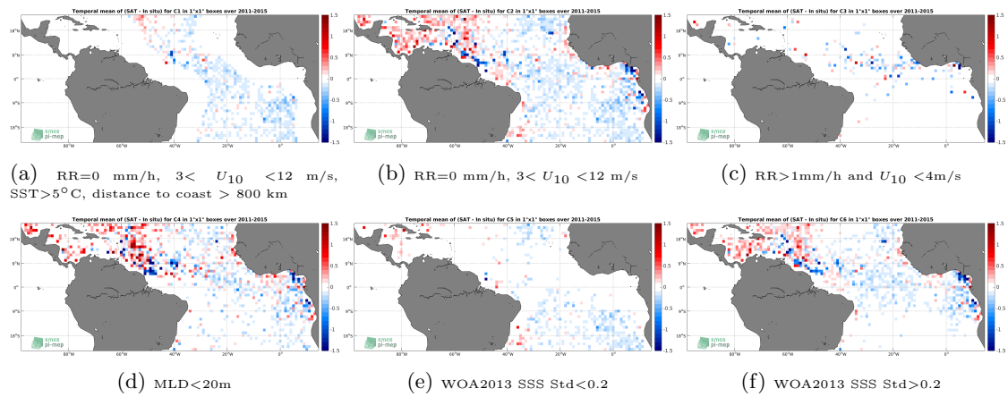
Figure 12: Temporal mean gridded over spatial boxes of size 1^\circ \times 1^\circ of \Delta SSS (Aquarius-L3-OR-V5-7DAY-RUNNING-1DEG - Argo) for 6 different subdatasets corresponding to:RR=0 mm/h, 3 < U_{10} < 12 m/s, SST >5^\circ C, distance to coast > 800 km (a), RR=0 mm/h, 3 < U_{10} < 12 m/s (b), RR >1 mm/h and U_{10} < 4 m/s (c),MLD <20 m (d),WOA2013 SSS Std <0.2 (e),WOA2013 SSS Std >0.2 (f).
