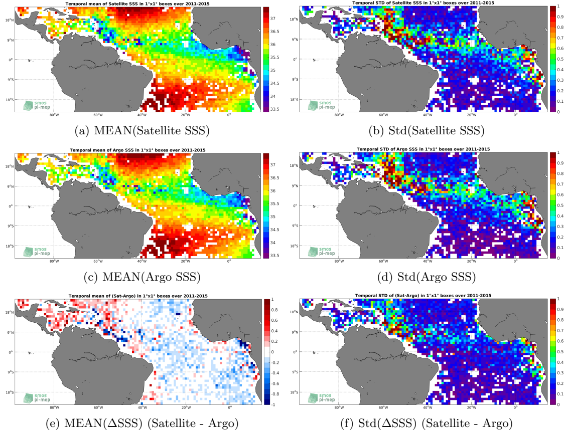
Figure 6: Temporal mean (left) and Std (right) of SSS from Aquarius-L3-OR-V5-7DAY-RUNNING-1DEG (top), Argo (middle), and of \Delta SSS (Satellite - Argo). Only match-up pairs are used to generate these maps.
