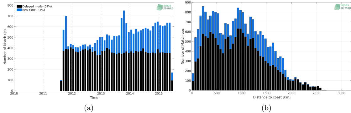
Figure 1: Number of match-ups between Argo and Aquarius-L3-OR-V5-7DAY-RUNNING-1DEG SSS as a function of time (a) and as function of the distance to coast (b) over the Tropical Atlantic Ocean Pi-MEP region and for the full satellite product period.
