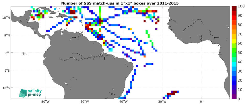
Figure 5: Number of SSS match-ups between TSG (SAMOS) SSS and the Aquarius SSS L3 OR v5 - 7-Day running - Rain mask (NASA-GSFC) SSS product for the Tropical Atlantic Ocean Pi-MEP region over 1^\circ \times 1^\circ boxes and for the full satellite product period.
