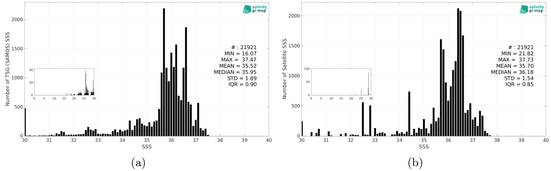
Figure 3: Histograms of SSS from TSG (SAMOS) (a) and Aquarius SSS L3 OR v5 - 7-Day running - Rain mask (NASA-GSFC) (b) considering all match-up pairs per bins of 0.1 over the Tropical Atlantic Ocean Pi-MEP region and for the full satellite product period.
