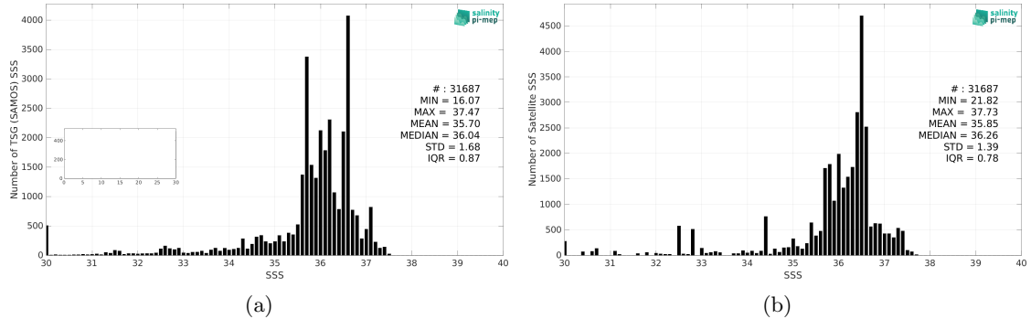
Figure 2: Histograms of SSS from TSG (SAMOS) (a) and Aquarius SSS L3 OR v5 - 7-Day running - Rain mask (NASA-GSFC) (b) considering all match-up pairs per bins of 0.1 over the Tropical Atlantic Ocean Pi-MEP region and for the full satellite product period.
