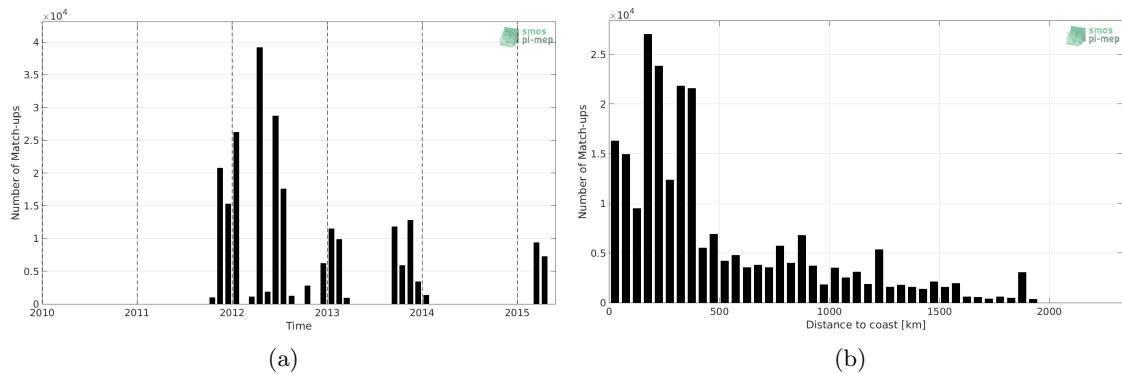
Figure 1: Number of match-ups between TSG-SAMOS and Aquarius-L3-OR-V5-7DAY-RUNNING-RAIN-MASK-1DEG SSS as a function of time (a) and as function of the distance to coast (b) over the Tropical Atlantic Ocean Pi-MEP region and for the full satellite product period.
