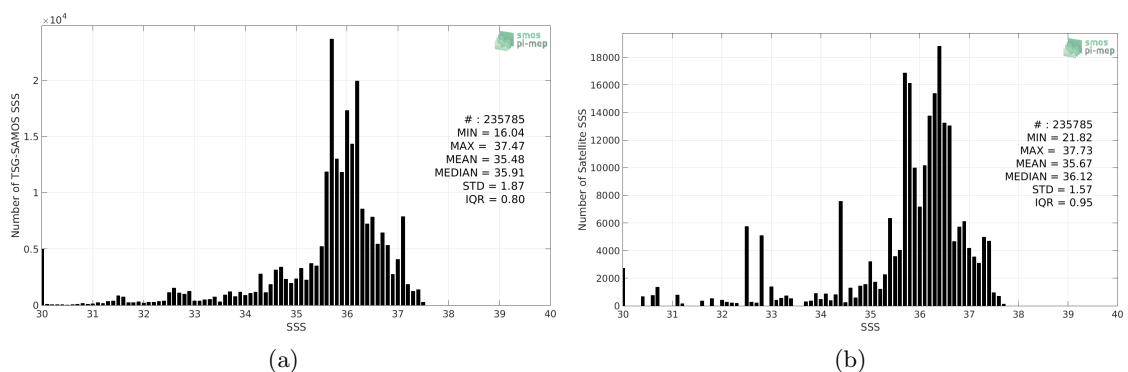
Figure 2: Histograms of SSS from TSG-SAMOS (a) and Aquarius-L3-OR-V5-7DAY-RUNNING-RAIN-MASK-1DEG (b) considering all match-up pairs per bins of 0.1 over the Tropical Atlantic Ocean Pi-MEP region and for the full satellite product period.
