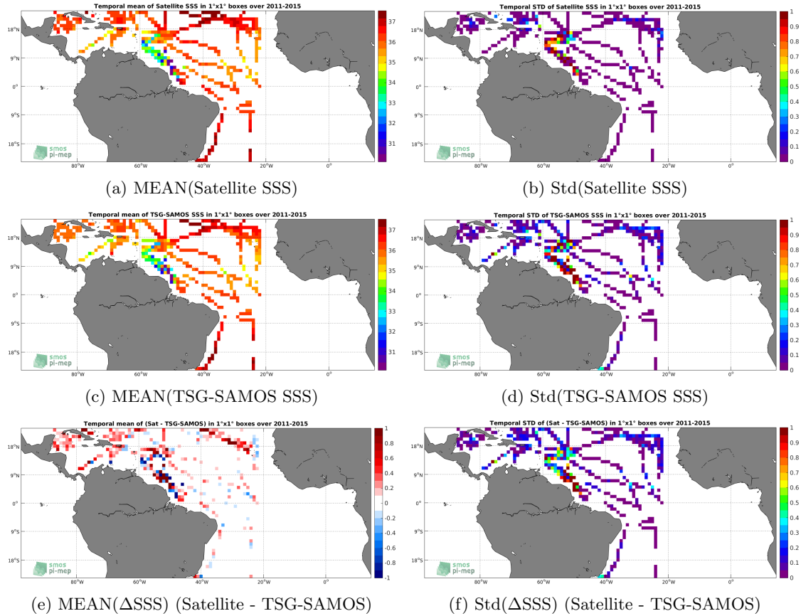
Figure 6: Temporal mean (left) and Std (right) of SSS from Aquarius-L3-OR-V5-7DAY-RUNNING-RAIN-MASK-1DEG (top), TSG-SAMOS (middle), and of \Delta SSS (Satellite - TSG-SAMOS). Only match-up pairs are used to generate these maps.
