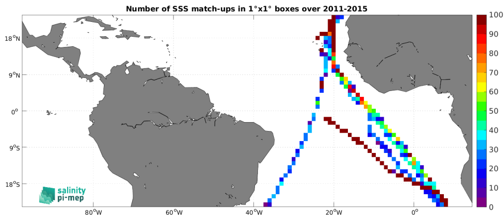
Figure 5: Number of SSS match-ups between TSG (Polarstern) SSS and the Aquarius SSS L3 OR v5 - 7-Day running - Rain mask (NASA-GSFC) SSS product for the Tropical Atlantic Ocean Pi-MEP region over 1^\circ \times 1^\circ boxes and for the full satellite product period.
