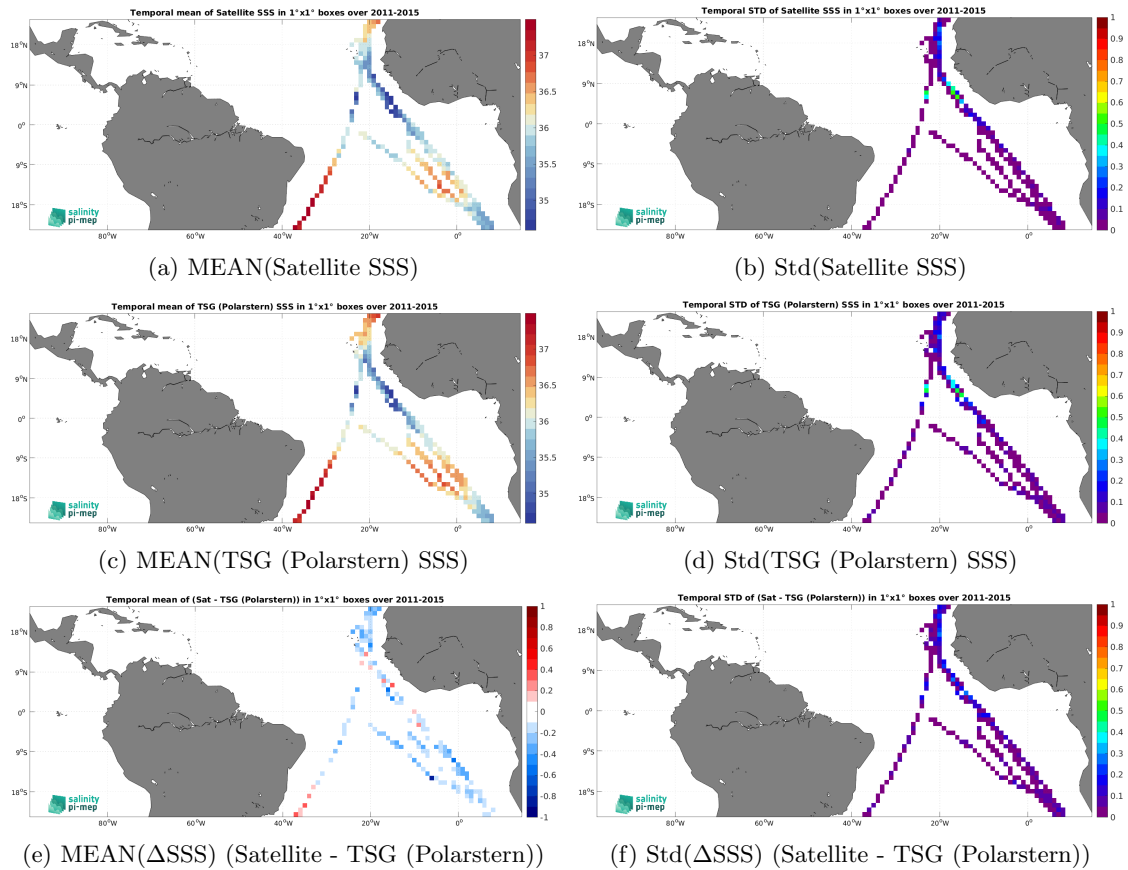
Figure 7: Temporal mean (left) and Std (right) of SSS from Aquarius SSS L3 OR v5 - 7-Day running - Rain mask (NASA-GSFC) (top), TSG (Polarstern) (middle), and of \Delta SSS (Satellite - TSG (Polarstern)). Only match-up pairs are used to generate these maps.
