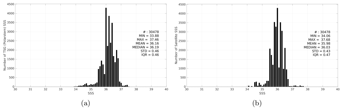
Figure 3: Histograms of SSS from TSG (Polarstern) (a) and Aquarius SSS L3 OR v5 - 7-Day running - Rain mask (NASA-GSFC) (b) considering all match-up pairs per bins of 0.1 over the Tropical Atlantic Ocean Pi-MEP region and for the full satellite product period.
