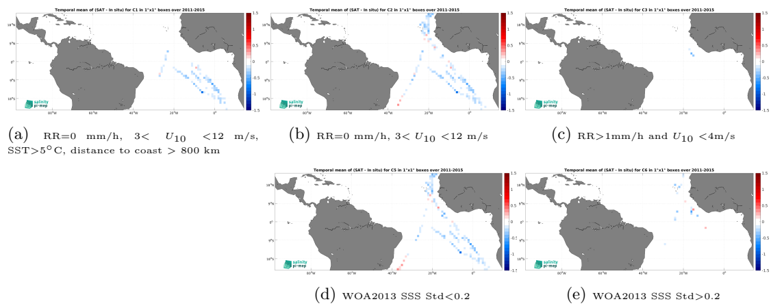
Figure 14: Temporal mean gridded over spatial boxes of size 1^\circ \times 1^\circ of \Delta\text{SSS} (Aquarius SSS L3 OR v5 - 7-Day running - Rain mask (NASA-GSFC) - TSG (Polarstern)) for 5 different subdatasets corresponding to:RR=0 mm/h, 3 < U_{10} < 12 m/s, SST >5^\circ\text{C} , distance to coast > 800 km (a), RR=0 mm/h, 3 < U_{10} < 12 m/s (b), RR >1 mm/h and U_{10} < 4 m/s (c), WOA2013 SSS Std <0.2 (d), WOA2013 SSS Std >0.2 (e).
