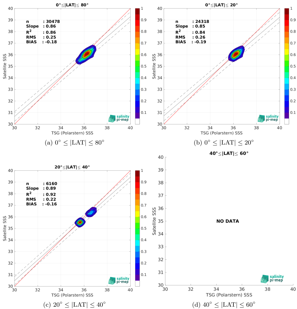
Figure 10: Contour maps of the concentration of Aquarius SSS L3 OR v5 - 7-Day running - Rain mask (NASA-GSFC) SSS (y-axis) versus TSG (Polarstern) SSS (x-axis) at match-up pairs for different latitude bands. For each plot, the red line shows x=y . The black thin and dashed lines indicate a linear fit through the data cloud and the \pm 95\% confidence levels, respectively. The number match-up pairs n , the slope and R^2 coefficient of the linear fit, the root mean square (RMS) and the mean bias between satellite and in situ data are indicated for each latitude band in each plots.
