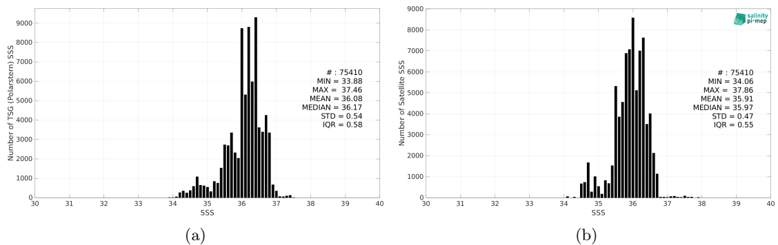
Figure 2: Histograms of SSS from TSG (Polarstern) (a) and Aquarius SSS L3 OR v5 - 7-Day running - Rain mask (NASA-GSFC) (b) considering all match-up pairs per bins of 0.1 over the Tropical Atlantic Ocean Pi-MEP region and for the full satellite product period.
