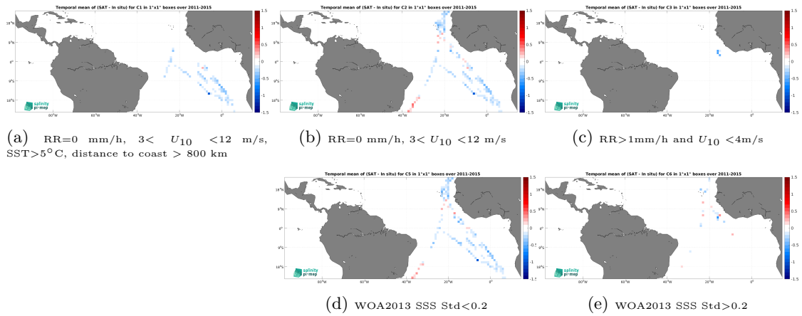
Figure 12: Temporal mean gridded over spatial boxes of size 1^{\circ}\times 1^{\circ} of \Delta\text{SSS} (Aquarius SSS L3 OR v5 - 7-Day running - Rain mask (NASA-GSFC) - TSG (Polarstern)) for 5 different subdatasets corresponding to:RR=0 mm/h, 3 < U_{10} < 12 m/s, SST > 5^{\circ}\text{C} , distance to coast > 800 km (a), RR=0 mm/h, 3 < U_{10} < 12 m/s (b), RR > 1 mm/h and U_{10} < 4 m/s (c), WOA2013 SSS Std < 0.2 (d), WOA2013 SSS Std > 0.2 (e).
