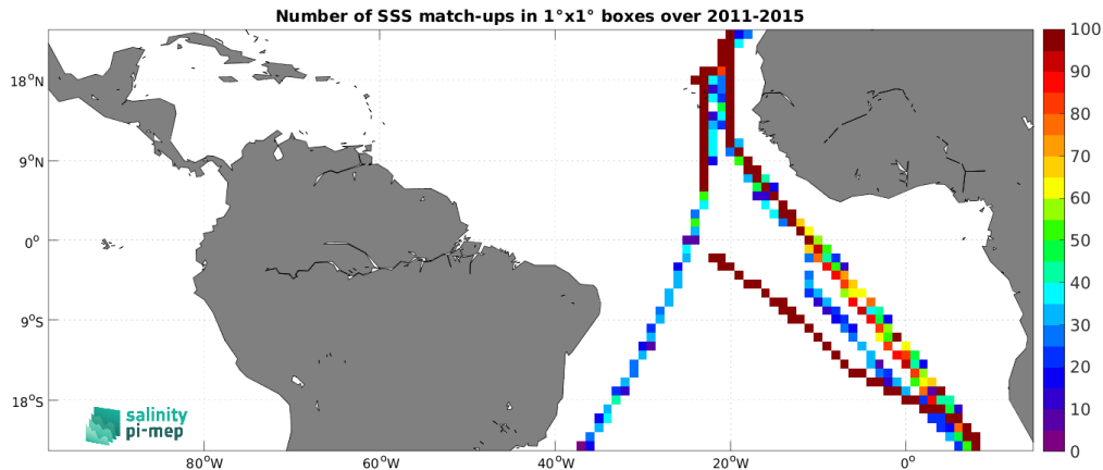
Figure 4: Number of SSS match-ups between TSG (Polarstern) SSS and the Aquarius SSS L3 OR v5 - 7-Day running - Rain mask (NASA-GSFC) SSS product for the Tropical Atlantic Ocean Pi-MEP region over 1^\circ \times 1^\circ boxes and for the full satellite product period.
