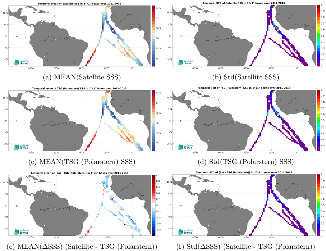
Figure 6: Temporal mean (left) and Std (right) of SSS from Aquarius SSS L3 OR v5 - 7-Day running - Rain mask (NASA-GSFC) (top), TSG (Polarstern) (middle), and of \Delta SSS (Satellite - TSG (Polarstern)). Only match-up pairs are used to generate these maps.
