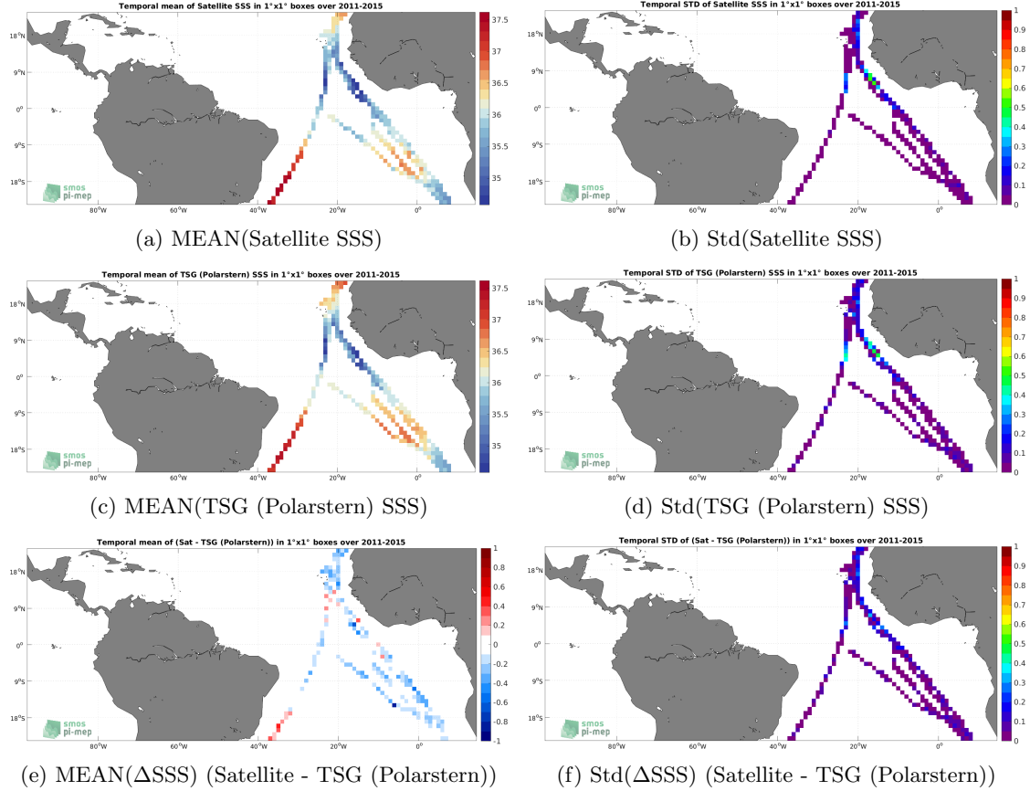
Figure 6: Temporal mean (left) and Std (right) of SSS from Aquarius SSS L3 OR v5 - 7-Day running - Rain mask (NASA-GSFC) (top), TSG (Polarstern) (middle), and of \Delta\text{SSS} (Satellite - TSG (Polarstern)). Only match-up pairs are used to generate these maps.
