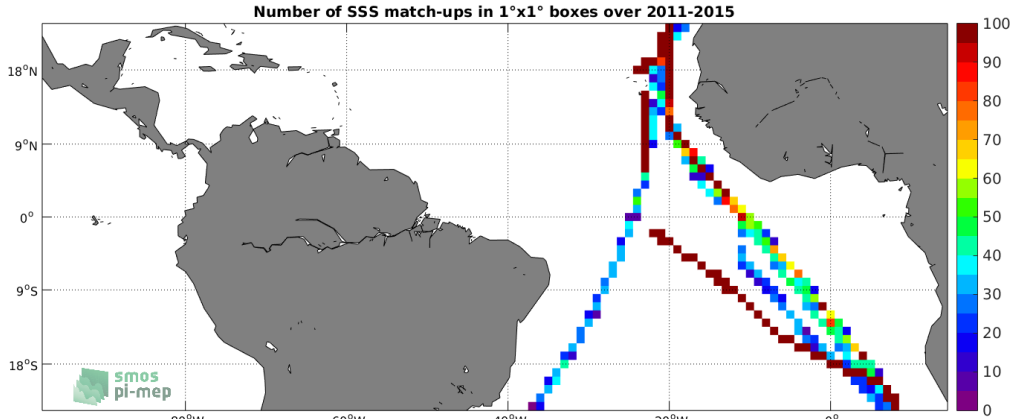
Figure 4: Number of SSS match-ups between TSG-POLARSTERN SSS and the Aquarius-L3-OR-V5-7DAY-RUNNING-RAIN-MASK-1DEG SSS product for the Tropical Atlantic Ocean Pi-MEP region over 1^\circ \times 1^\circ boxes and for the full satellite product period.
