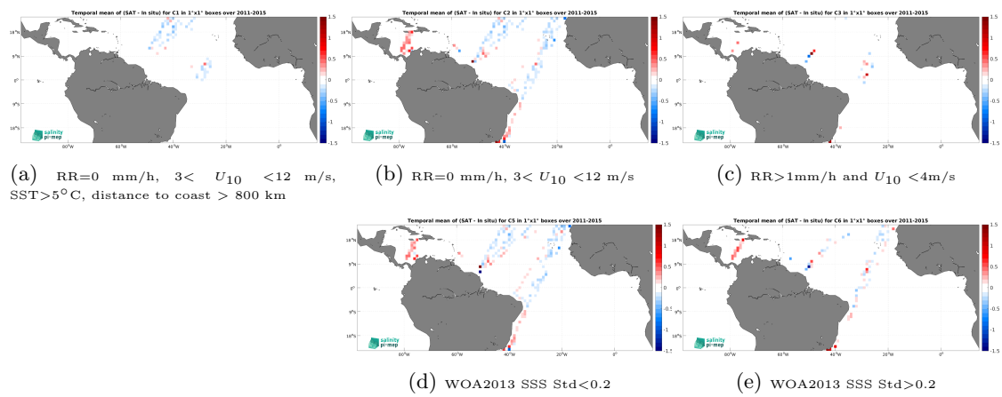
Figure 14: Temporal mean gridded over spatial boxes of size 1^\circ \times 1^\circ of \Delta SSS (Aquarius SSS L3 OR v5 - 7-Day running - Rain mask (NASA-GSFC) - TSG (LEGOS-DM)) for 5 different subdatasets corresponding to:RR=0 mm/h, 3 < U_{10} < 12 m/s, SST >5^\circ C, distance to coast > 800 km (a), RR=0 mm/h, 3 < U_{10} < 12 m/s (b), RR >1 mm/h and U_{10} < 4 m/s (c), WOA2013 SSS Std <0.2 (d), WOA2013 SSS Std >0.2 (e).
