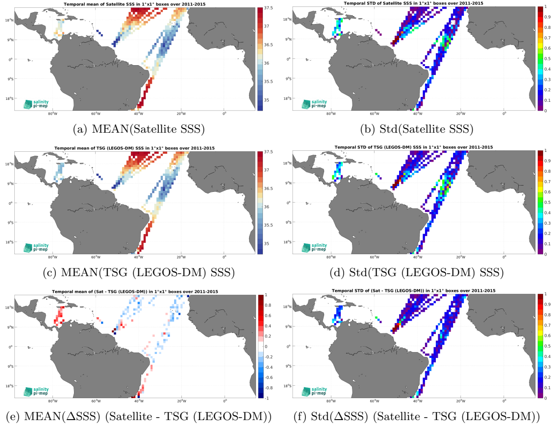
Figure 7: Temporal mean (left) and Std (right) of SSS from Aquarius SSS L3 OR v5 - 7-Day running - Rain mask (NASA-GSFC) (top), TSG (LEGOS-DM) (middle), and of \Delta\text{SSS} (Satellite - TSG (LEGOS-DM)). Only match-up pairs are used to generate these maps.
