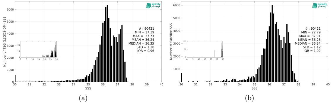
Figure 3: Histograms of SSS from TSG (LEGOS-DM) (a) and Aquarius SSS L3 OR v5 - 7-Day running - Rain mask (NASA-GSFC) (b) considering all match-up pairs per bins of 0.1 over the Tropical Atlantic Ocean Pi-MEP region and for the full satellite product period.
