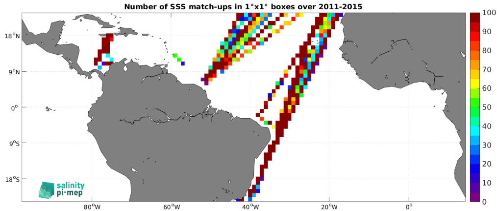
Figure 5: Number of SSS match-ups between TSG (LEGOS-DM) SSS and the Aquarius SSS L3 OR v5 - 7-Day running - Rain mask (NASA-GSFC) SSS product for the Tropical Atlantic Ocean Pi-MEP region over 1^\circ \times 1^\circ boxes and for the full satellite product period.
