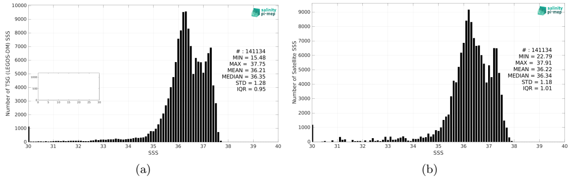
Figure 2: Histograms of SSS from TSG (LEGOS-DM) (a) and Aquarius SSS L3 OR v5 - 7-Day running - Rain mask (NASA-GSFC) (b) considering all match-up pairs per bins of 0.1 over the Tropical Atlantic Ocean Pi-MEP region and for the full satellite product period.
