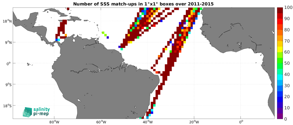
Figure 4: Number of SSS match-ups between TSG (LEGOS-DM) SSS and the Aquarius SSS L3 OR v5 - 7-Day running - Rain mask (NASA-GSFC) SSS product for the Tropical Atlantic Ocean Pi-MEP region over 1^\circ \times 1^\circ boxes and for the full satellite product period.
