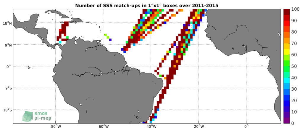
Figure 4: Number of SSS match-ups between TSG-LEGOS-DM SSS and the Aquarius-L3-OR-V5-7DAY-RUNNING-RAIN-MASK-1DEG SSS product for the Tropical Atlantic Ocean Pi-MEP region over 1^\circ \times 1^\circ boxes and for the full satellite product period.
