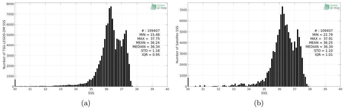
Figure 2: Histograms of SSS from TSG-LEGOS-DM (a) and Aquarius-L3-OR-V5-7DAY-RUNNING-RAIN-MASK-1DEG (b) considering all match-up pairs per bins of 0.1 over the Tropical Atlantic Ocean Pi-MEP region and for the full satellite product period.
