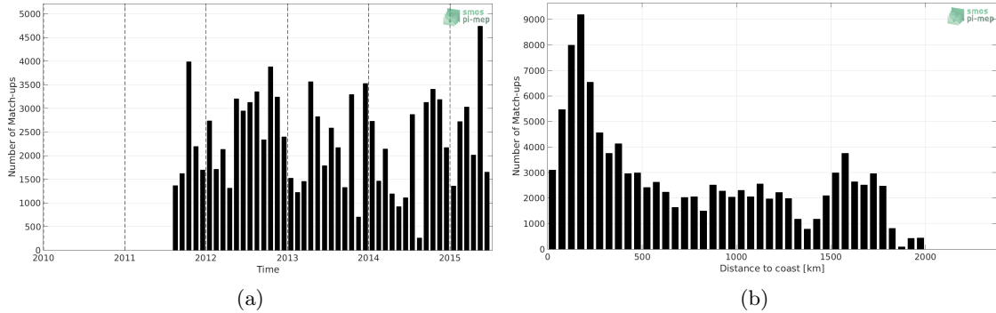
Figure 1: Number of match-ups between TSG-LEGOS-DM and Aquarius-L3-OR-V5-7DAY-RUNNING-RAIN-MASK-1DEG SSS as a function of time (a) and as function of the distance to coast (b) over the Tropical Atlantic Ocean Pi-MEP region and for the full satellite product period.
