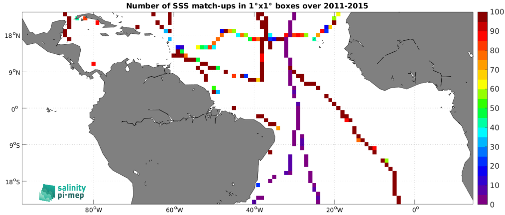
Figure 5: Number of SSS match-ups between TSG (GOSUD-Sailing-ship) SSS and the Aquarius SSS L3 OR v5 - 7-Day running - Rain mask (NASA-GSFC) SSS product for the Tropical Atlantic Ocean Pi-MEP region over 1^\circ \times 1^\circ boxes and for the full satellite product period.
