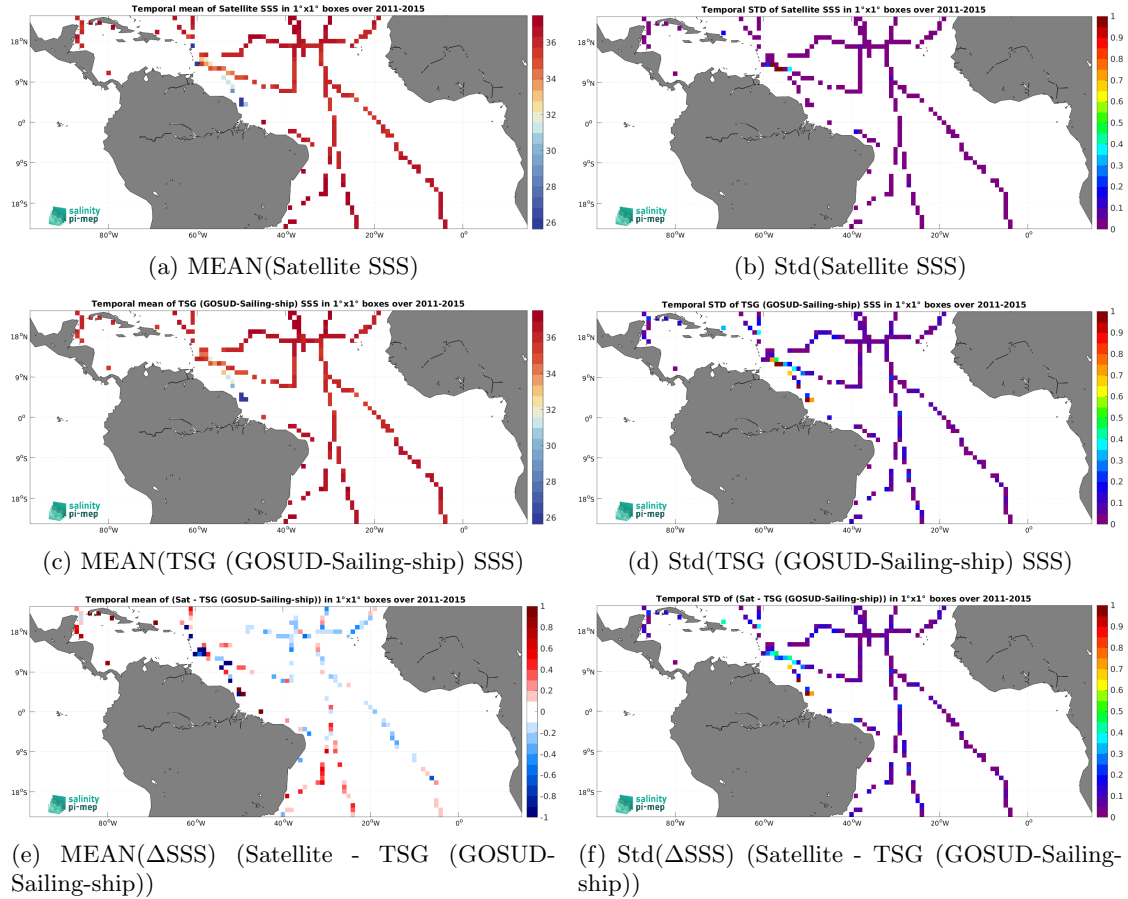
Figure 7: Temporal mean (left) and Std (right) of SSS from Aquarius SSS L3 OR v5 - 7-Day running - Rain mask (NASA-GSFC) (top), TSG (GOSUD-Sailing-ship) (middle), and of \Delta\text{SSS} (Satellite - TSG (GOSUD-Sailing-ship)). Only match-up pairs are used to generate these maps.
