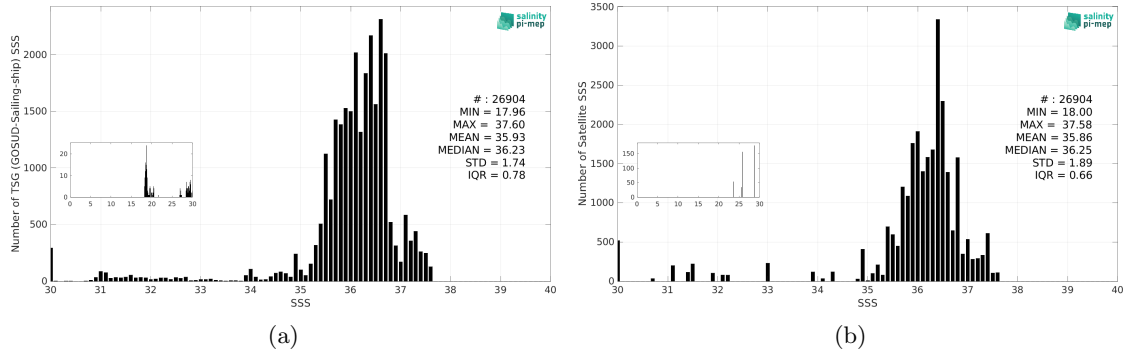
Figure 3: Histograms of SSS from TSG (GOSUD-Sailing-ship) (a) and Aquarius SSS L3 OR v5 - 7-Day running - Rain mask (NASA-GSFC) (b) considering all match-up pairs per bins of 0.1 over the Tropical Atlantic Ocean Pi-MEP region and for the full satellite product period.
