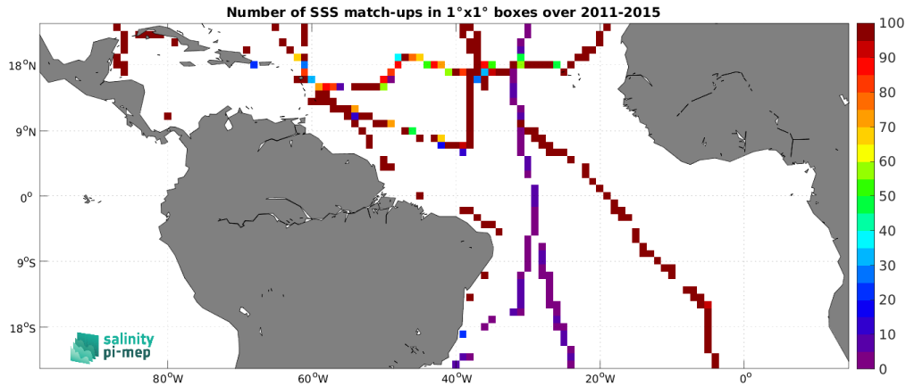
Figure 4: Number of SSS match-ups between TSG (GOSUD-Sailing-ship) SSS and the Aquarius SSS L3 OR v5 - 7-Day running - Rain mask (NASA-GSFC) SSS product for the Tropical Atlantic Ocean Pi-MEP region over 1^\circ \times 1^\circ boxes and for the full satellite product period.
