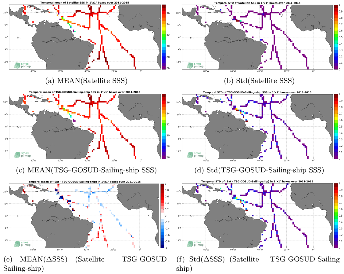
Figure 6: Temporal mean (left) and Std (right) of SSS from Aquarius-L3-OR-V5-7DAY-RUNNING-RAIN-MASK-1DEG (top), TSG-GOSUD-Sailing-ship (middle), and of \Delta SSS (Satellite - TSG-GOSUD-Sailing-ship). Only match-up pairs are used to generate these maps.
