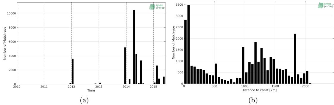
Figure 1: Number of match-ups between TSG-GOSUD-Sailing-ship and Aquarius-L3-OR-V5-7DAY-RUNNING-RAIN-MASK-1DEG SSS as a function of time (a) and as function of the distance to coast (b) over the Tropical Atlantic Ocean Pi-MEP region and for the full satellite product period.
