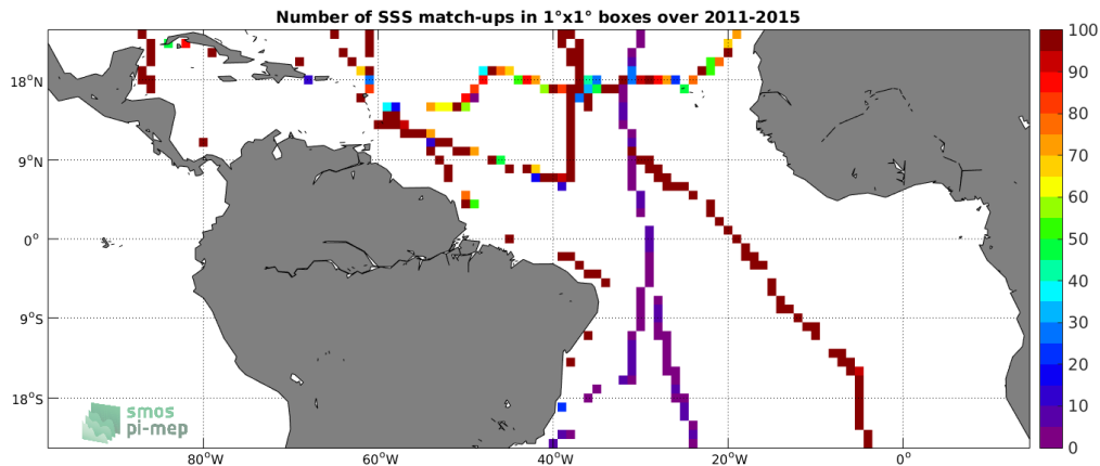
Figure 4: Number of SSS match-ups between TSG-GOSUD-Sailing-ship SSS and the Aquarius-L3-OR-V5-7DAY-RUNNING-RAIN-MASK-1DEG SSS product for the Tropical Atlantic Ocean Pi-MEP region over 1°x1° boxes and for the full satellite product period.
