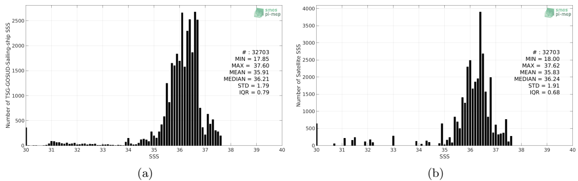
Figure 2: Histograms of SSS from TSG-GOSUD-Sailing-ship (a) and Aquarius-L3-OR-V5-7DAY-RUNNING-RAIN-MASK-1DEG (b) considering all match-up pairs per bins of 0.1 over the Tropical Atlantic Ocean Pi-MEP region and for the full satellite product period.
