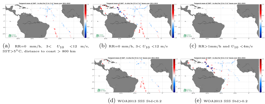
Figure 12: Temporal mean gridded over spatial boxes of size 1^\circ \times 1^\circ of \Delta SSS (Aquarius-L3-OR-V5-7DAY-RUNNING-RAIN-MASK-1DEG - TSG-GOSUD-Sailing-ship) for 5 different subdatasets corresponding to:RR=0 mm/h, 3 < U_{10} < 12 m/s, SST >5^\circ\text{C} , distance to coast > 800 km (a), RR=0 mm/h, 3 < U_{10} < 12 m/s (b), RR >1 mm/h and U_{10} < 4 m/s (c), WOA2013 SSS Std <0.2 (d), WOA2013 SSS Std >0.2 (e).
