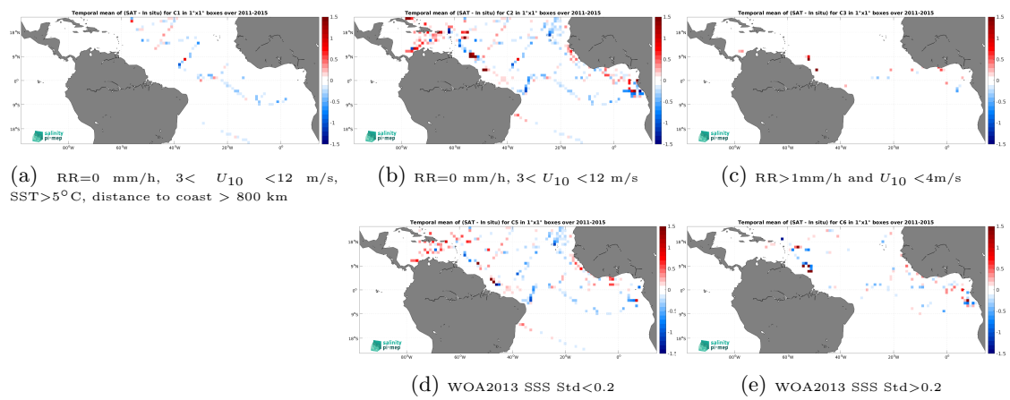
Figure 14: Temporal mean gridded over spatial boxes of size 1^\circ \times 1^\circ of \Delta SSS (Aquarius SSS L3 OR v5 - 7-Day running - Rain mask (NASA-GSFC) - TSG (GOSUD-Research-vessel)) for 5 different subdatasets corresponding to:RR=0 mm/h, 3 < U_{10} < 12 m/s, SST >5^\circ\text{C} , distance to coast > 800 km (a), RR=0 mm/h, 3 < U_{10} < 12 m/s (b), RR >1 mm/h and U_{10} < 4 m/s (c), WOA2013 SSS Std <0.2 (d), WOA2013 SSS Std >0.2 (e).
