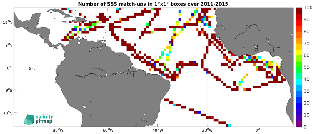
Figure 5: Number of SSS match-ups between TSG (GOSUD-Research-vessel) SSS and the Aquarius SSS L3 OR v5 - 7-Day running - Rain mask (NASA-GSFC) SSS product for the Tropical Atlantic Ocean Pi-MEP region over 1^\circ \times 1^\circ boxes and for the full satellite product period.
