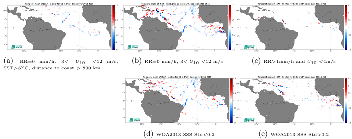
Figure 12: Temporal mean gridded over spatial boxes of size 1^\circ \times 1^\circ of \Delta SSS (Aquarius SSS L3 OR v5 - 7-Day running - Rain mask (NASA-GSFC) - TSG (GOSUD-Research-vessel)) for 5 different subdatasets corresponding to:RR=0 mm/h, 3 < U_{10} < 12 m/s, SST >5^\circ\text{C} , distance to coast > 800 km (a), RR=0 mm/h, 3 < U_{10} < 12 m/s (b), RR >1 mm/h and U_{10} < 4 m/s (c), WOA2013 SSS Std <0.2 (d), WOA2013 SSS Std >0.2 (e).
