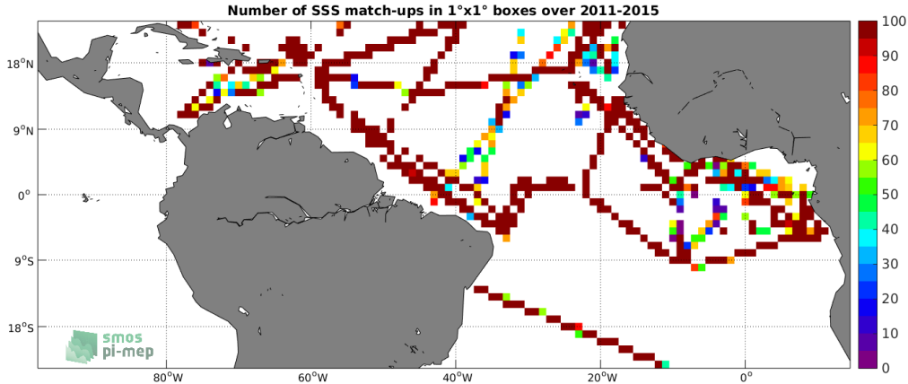
Figure 4: Number of SSS match-ups between TSG-GOSUD-Research-vessel SSS and the Aquarius-L3-OR-V5-7DAY-RUNNING-RAIN-MASK-1DEG SSS product for the Tropical Atlantic Ocean Pi-MEP region over 1^\circ \times 1^\circ boxes and for the full satellite product period.
