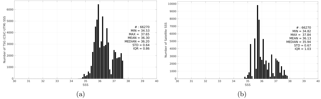
Figure 3: Histograms of SSS from TSG (CSIC-UTM) (a) and Aquarius SSS L3 OR v5 - 7-Day running - Rain mask (NASA-GSFC) (b) considering all match-up pairs per bins of 0.1 over the Tropical Atlantic Ocean Pi-MEP region and for the full satellite product period.
