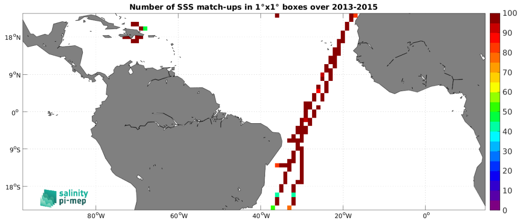
Figure 5: Number of SSS match-ups between TSG (CSIC-UTM) SSS and the Aquarius SSS L3 OR v5 - 7-Day running - Rain mask (NASA-GSFC) SSS product for the Tropical Atlantic Ocean Pi-MEP region over 1^\circ \times 1^\circ boxes and for the full satellite product period.
