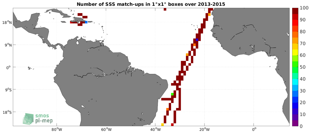
Figure 4: Number of SSS match-ups between TSG (CSIC-UTM) SSS and the Aquarius SSS L3 OR v5 - 7-Day running - Rain mask (NASA-GSFC) SSS product for the Tropical Atlantic Ocean Pi-MEP region over 1^\circ \times 1^\circ boxes and for the full satellite product period.
