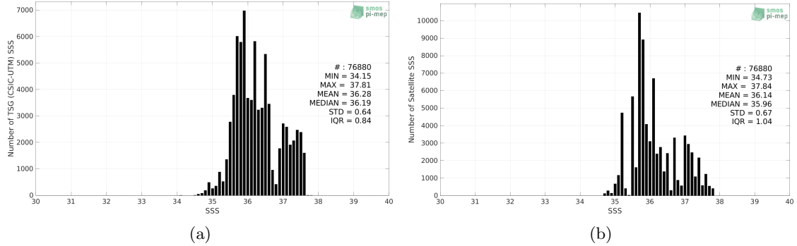
Figure 2: Histograms of SSS from TSG (CSIC-UTM) (a) and Aquarius SSS L3 OR v5 - 7-Day running - Rain mask (NASA-GSFC) (b) considering all match-up pairs per bins of 0.1 over the Tropical Atlantic Ocean Pi-MEP region and for the full satellite product period.
