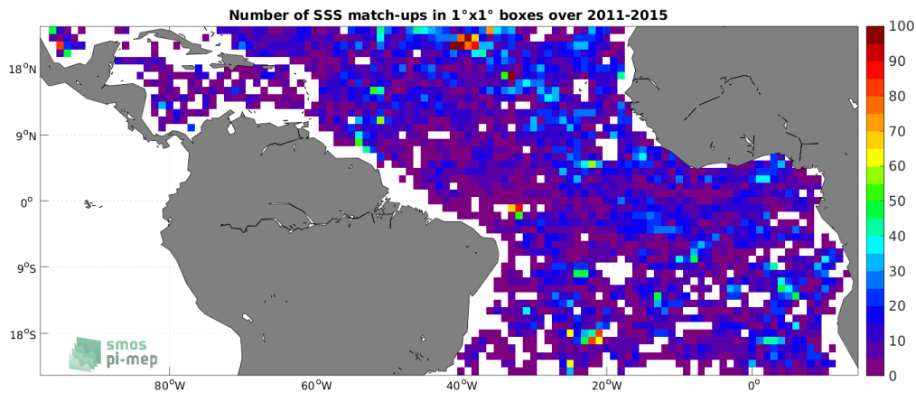
Figure 4: Number of SSS match-ups between Argo SSS and the Aquarius SSS L3 OR v5 - 7-Day running - Rain mask (NASA-GSFC) SSS product for the Tropical Atlantic Ocean Pi-MEP region over 1^\circ \times 1^\circ boxes and for the full satellite product period.
