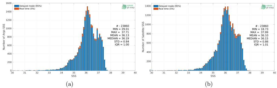
Figure 2: Histograms of SSS from Argo (a) and Aquarius SSS L3 OR v5 - 7-Day running - Rain mask (NASA-GSFC) (b) considering all match-up pairs per bins of 0.1 over the Tropical Atlantic Ocean Pi-MEP region and for the full satellite product period.
