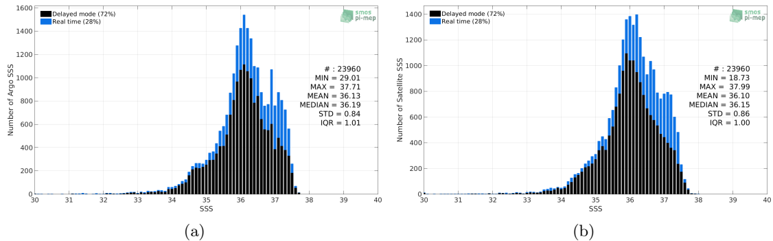
Figure 2: Histograms of SSS from Argo (a) and Aquarius-L3-OR-V5-7DAY-RUNNING-RAIN-MASK-1DEG (b) considering all match-up pairs per bins of 0.1 over the Tropical Atlantic Ocean Pi-MEP region and for the full satellite product period.
