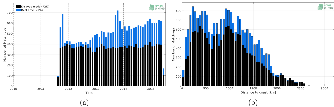
Figure 1: Number of match-ups between Argo and Aquarius-L3-OR-V5-7DAY-RUNNING-RAIN-MASK-1DEG SSS as a function of time (a) and as function of the distance to coast (b) over the Tropical Atlantic Ocean Pi-MEP region and for the full satellite product period.
