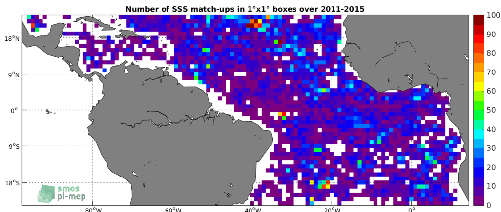
Figure 4: Number of SSS match-ups between Argon SSS and the Aquarius-L3-OR-V5-7DAY-RUNNING-RAIN-MASK-1DEG SSS product for the Tropical Atlantic Ocean Pi-MEP region over 1°x1° boxes and for the full satellite product period.
