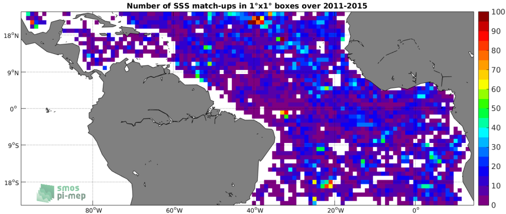
Figure 4: Number of SSS match-ups between Argo SSS and the Aquarius-L3-OR-V5-7DAY-RUNNING-RAIN-MASK-1DEG SSS product for the Tropical Atlantic Ocean Pi-MEP region over 1^\circ \times 1^\circ boxes and for the full satellite product period.
