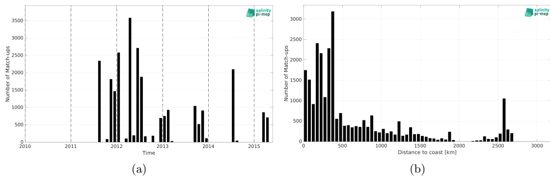
Figure 2: Number of match-ups between TSG (SAMOS) and Aquarius SSS L3 OR v5 - Monthly (NASA-GSFC) SSS as a function of time (a) and as function of the distance to coast (b) over the Tropical Atlantic Ocean Pi-MEP region and for the full satellite product period.
