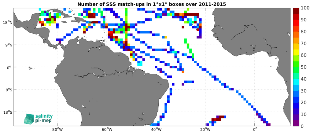
Figure 5: Number of SSS match-ups between TSG (SAMOS) SSS and the Aquarius SSS L3 OR v5 - Monthly (NASA-GSFC) SSS product for the Tropical Atlantic Ocean Pi-MEP region over 1^\circ \times 1^\circ boxes and for the full satellite product period.
