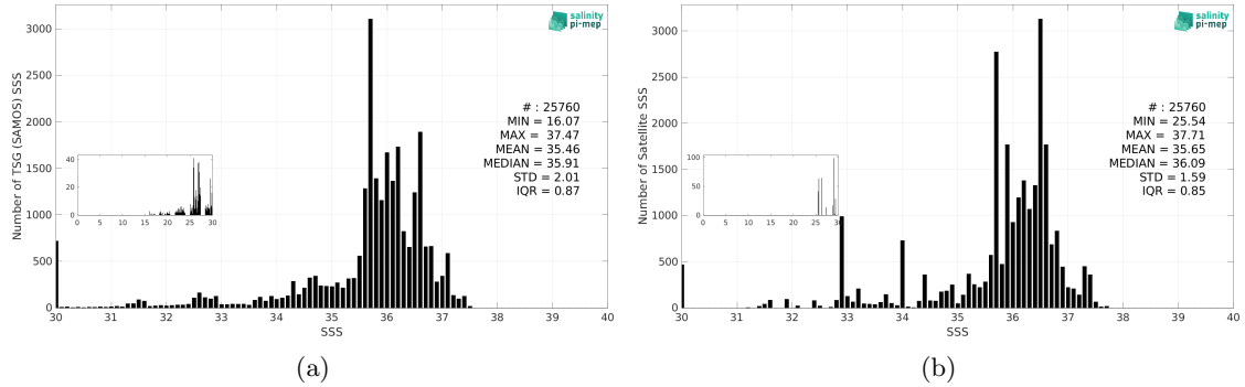
Figure 3: Histograms of SSS from TSG (SAMOS) (a) and Aquarius SSS L3 OR v5 - Monthly (NASA-GSFC) (b) considering all match-up pairs per bins of 0.1 over the Tropical Atlantic Ocean Pi-MEP region and for the full satellite product period.
