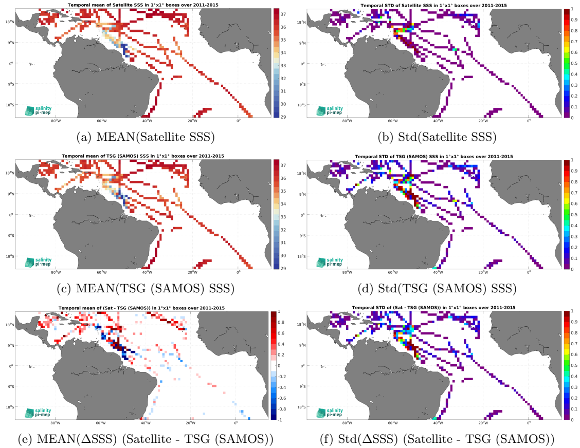
Figure 7: Temporal mean (left) and Std (right) of SSS from Aquarius SSS L3 OR v5 - Monthly (NASA-GSFC) (top), TSG (SAMOS) (middle), and of \Delta\text{SSS} (Satellite - TSG (SAMOS)). Only match-up pairs are used to generate these maps.
