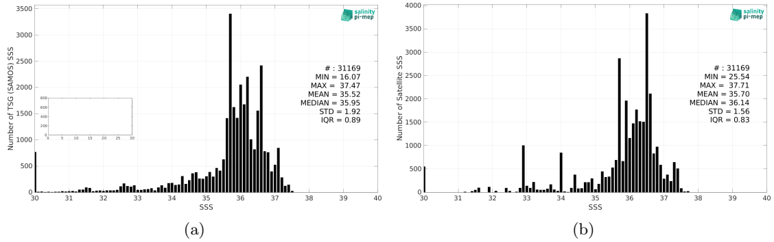
Figure 2: Histograms of SSS from TSG (SAMOS) (a) and Aquarius SSS L3 OR v5 - Monthly (NASA-GSFC) (b) considering all match-up pairs per bins of 0.1 over the Tropical Atlantic Ocean Pi-MEP region and for the full satellite product period.
