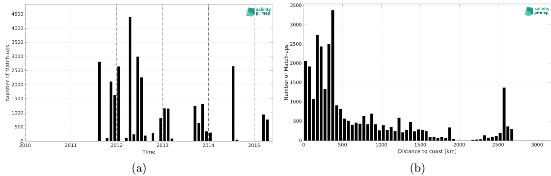
Figure 1: Number of match-ups between TSG (SAMOS) and Aquarius SSS L3 OR v5 - Monthly (NASA-GSFC) SSS as a function of time (a) and as function of the distance to coast (b) over the Tropical Atlantic Ocean Pi-MEP region and for the full satellite product period.
