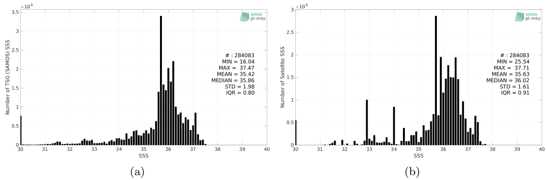
Figure 2: Histograms of SSS from TSG (SAMOS) (a) and Aquarius SSS L3 OR v5 - Monthly (NASA-GSFC) (b) considering all match-up pairs per bins of 0.1 over the Tropical Atlantic Ocean Pi-MEP region and for the full satellite product period.
