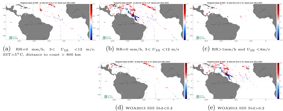
Figure 12: Temporal mean gridded over spatial boxes of size 1^\circ \times 1^\circ of \Delta\text{SSS} (Aquarius SSS L3 OR v5 - Monthly (NASA-GSFC) - TSG (SAMOS)) for 5 different subdatasets corresponding to:RR=0 mm/h, 3 < U_{10} < 12 m/s, SST >5^\circ\text{C} , distance to coast > 800 km (a), RR=0 mm/h, 3 < U_{10} < 12 m/s (b), RR >1 mm/h and U_{10} < 4 m/s (c), WOA2013 SSS Std <0.2 (d), WOA2013 SSS Std >0.2 (e).
