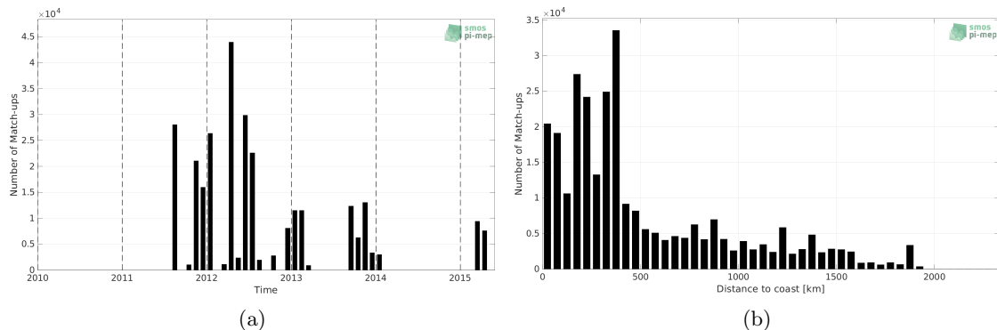
Figure 1: Number of match-ups between TSG (SAMOS) and Aquarius SSS L3 OR v5 - Monthly (NASA-GSFC) SSS as a function of time (a) and as function of the distance to coast (b) over the Tropical Atlantic Ocean Pi-MEP region and for the full satellite product period.
