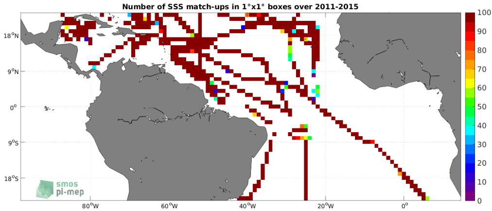
Figure 4: Number of SSS match-ups between TSG (SAMOS) SSS and the Aquarius SSS L3 OR v5 - Monthly (NASA-GSFC) SSS product for the Tropical Atlantic Ocean Pi-MEP region over 1^\circ \times 1^\circ boxes and for the full satellite product period.
