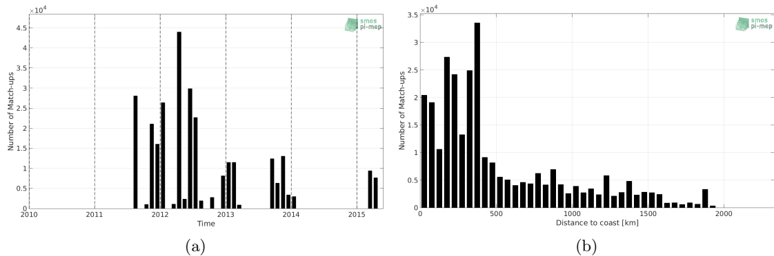
Figure 1: Number of match-ups between TSG-SAMOS and Aquarius-L3-OR-V5-MONTHLY-1DEG SSS as a function of time (a) and as function of the distance to coast (b) over the Tropical Atlantic Ocean Pi-MEP region and for the full satellite product period.
