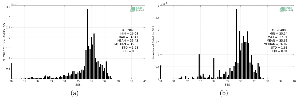
Figure 2: Histograms of SSS from TSG-SAMOS (a) and Aquarius-L3-OR-V5-MONTHLY-1DEG (b) considering all match-up pairs per bins of 0.1 over the Tropical Atlantic Ocean Pi-MEP region and for the full satellite product period.
