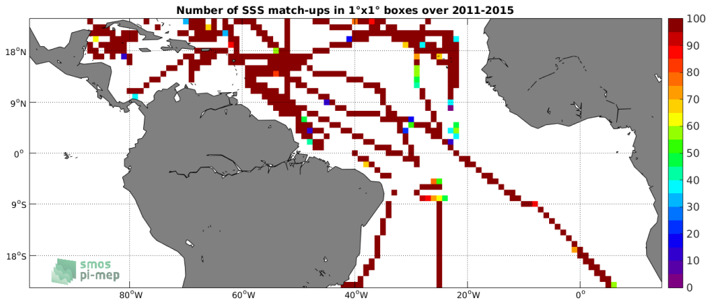
Figure 4: Number of SSS match-ups between TSG-SAMOS SSS and the Aquarius-L3-OR-V5-MONTHLY-1DEG SSS product for the Tropical Atlantic Ocean Pi-MEP region over 1^\circ \times 1^\circ boxes and for the full satellite product period.
