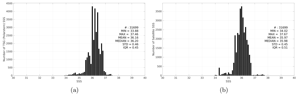
Figure 3: Histograms of SSS from TSG (Polarstern) (a) and Aquarius SSS L3 OR v5 - Monthly (NASA-GSFC) (b) considering all match-up pairs per bins of 0.1 over the Tropical Atlantic Ocean Pi-MEP region and for the full satellite product period.
