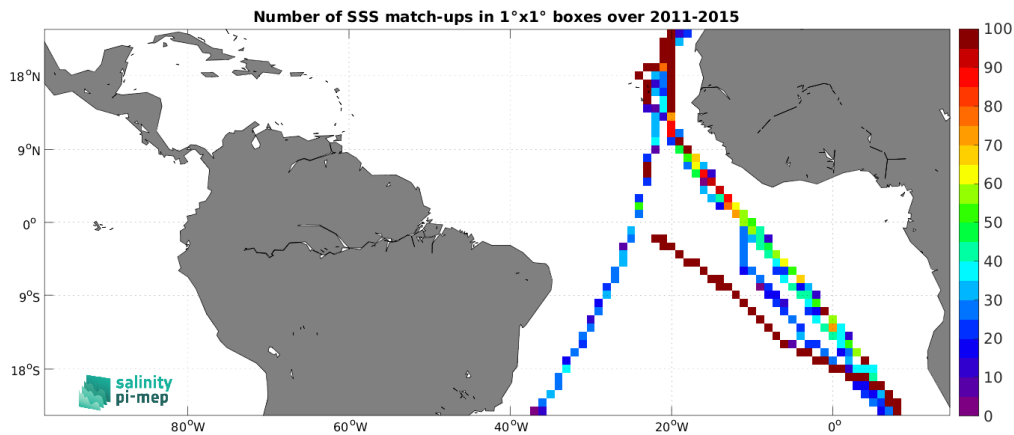
Figure 5: Number of SSS match-ups between TSG (Polarstern) SSS and the Aquarius SSS L3 OR v5 - Monthly (NASA-GSFC) SSS product for the Tropical Atlantic Ocean Pi-MEP region over 1^\circ \times 1^\circ boxes and for the full satellite product period.
