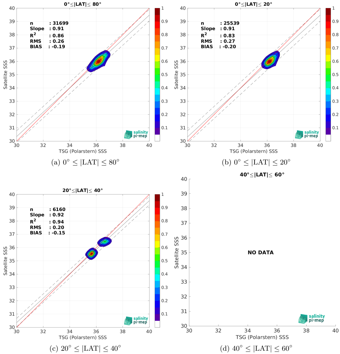
Figure 10: Contour maps of the concentration of Aquarius SSS L3 OR v5 - Monthly (NASA-GSFC) SSS (y-axis) versus TSG (Polarstern) SSS (x-axis) at match-up pairs for different latitude bands. For each plot, the red line shows x=y . The black thin and dashed lines indicate a linear fit through the data cloud and the \pm 95\% confidence levels, respectively. The number match-up pairs n , the slope and R^2 coefficient of the linear fit, the root mean square (RMS) and the mean bias between satellite and in situ data are indicated for each latitude band in each plots.
