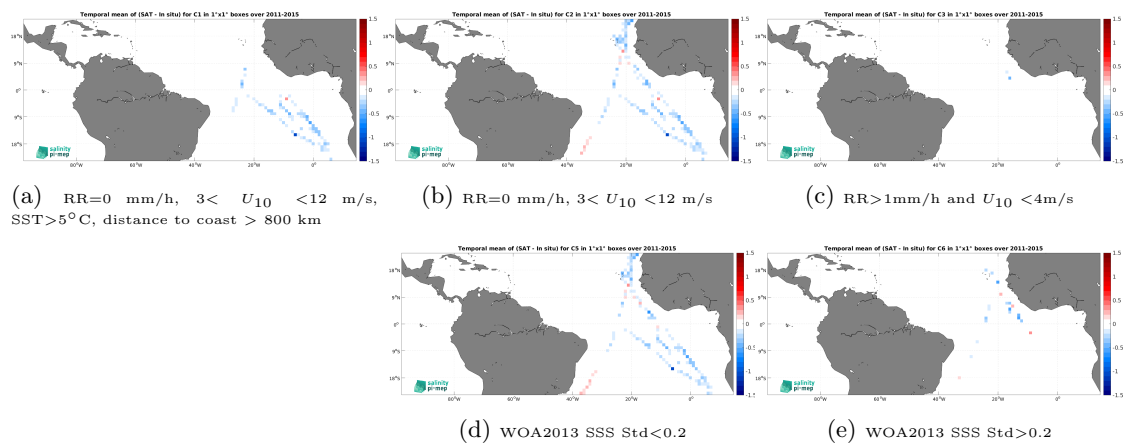
Figure 14: Temporal mean gridded over spatial boxes of size 1^\circ \times 1^\circ of \Delta SSS (Aquarius SSS L3 OR v5 - Monthly (NASA-GSFC) - TSG (Polarstern)) for 5 different subdatasets corresponding to:RR=0 mm/h, 3 < U_{10} < 12 m/s, SST >5^\circ\text{C} , distance to coast > 800 km (a), RR=0 mm/h, 3 < U_{10} < 12 m/s (b), RR >1 mm/h and U_{10} < 4 m/s (c), WOA2013 SSS Std <0.2 (d), WOA2013 SSS Std >0.2 (e).
