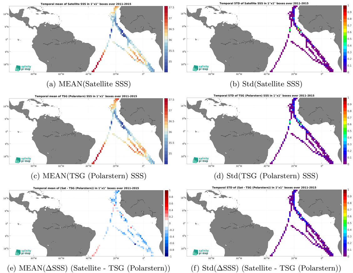
Figure 7: Temporal mean (left) and Std (right) of SSS from Aquarius SSS L3 OR v5 - Monthly (NASA-GSFC) (top), TSG (Polarstern) (middle), and of \Delta SSS (Satellite - TSG (Polarstern)). Only match-up pairs are used to generate these maps.
