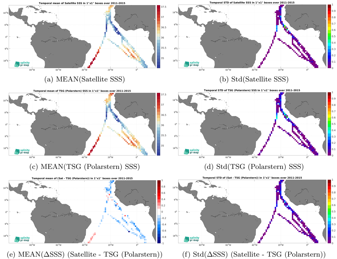
Figure 6: Temporal mean (left) and Std (right) of SSS from Aquarius SSS L3 OR v5 - Monthly (NASA-GSFC) (top), TSG (Polarstern) (middle), and of \Delta SSS (Satellite - TSG (Polarstern)). Only match-up pairs are used to generate these maps.
