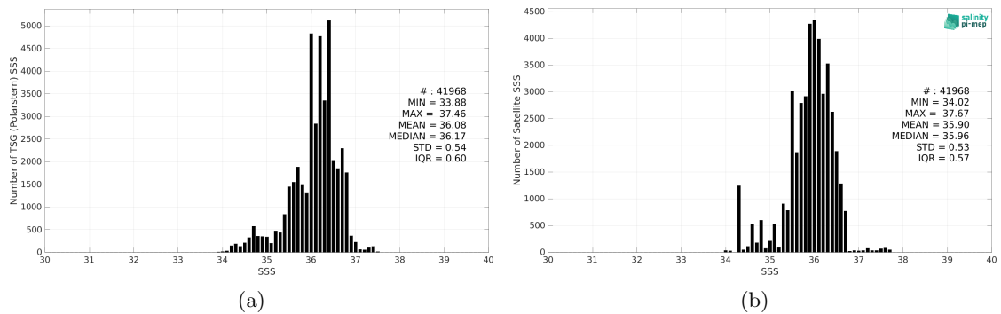
Figure 2: Histograms of SSS from TSG (Polarstern) (a) and Aquarius SSS L3 OR v5 - Monthly (NASA-GSFC) (b) considering all match-up pairs per bins of 0.1 over the Tropical Atlantic Ocean Pi-MEP region and for the full satellite product period.
