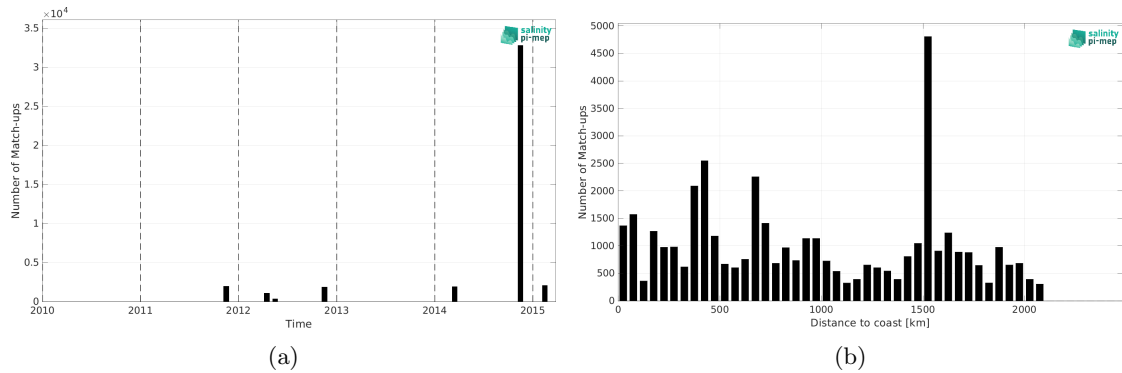
Figure 1: Number of match-ups between TSG (Polarstern) and Aquarius SSS L3 OR v5 - Monthly (NASA-GSFC) SSS as a function of time (a) and as function of the distance to coast (b) over the Tropical Atlantic Ocean Pi-MEP region and for the full satellite product period.
