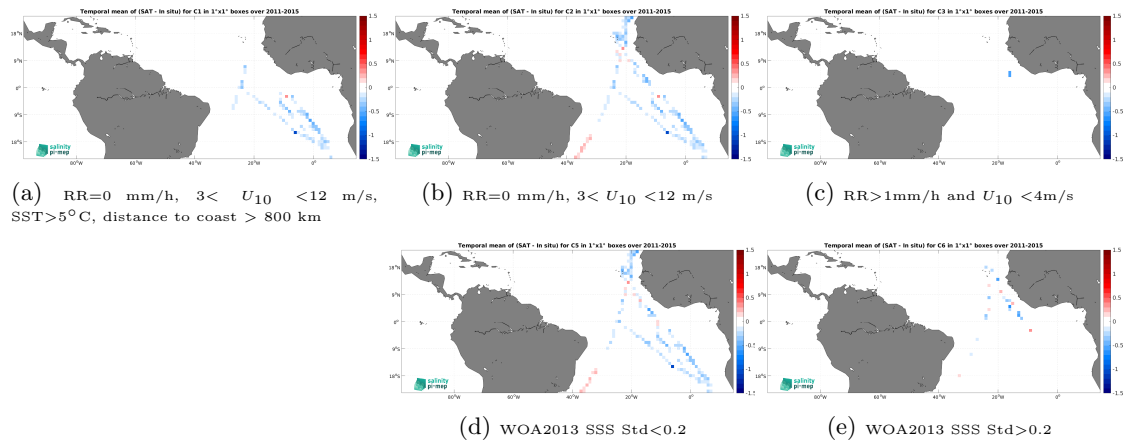
Figure 12: Temporal mean gridded over spatial boxes of size 1^\circ \times 1^\circ of \Delta SSS (Aquarius SSS L3 OR v5 - Monthly (NASA-GSFC) - TSG (Polarstern)) for 5 different subdatasets corresponding to:RR=0 mm/h, 3 < U_{10} < 12 m/s, SST >5^\circ\text{C} , distance to coast > 800 km (a), RR=0 mm/h, 3 < U_{10} < 12 m/s (b), RR >1 mm/h and U_{10} < 4 m/s (c), WOA2013 SSS Std <0.2 (d), WOA2013 SSS Std >0.2 (e).
