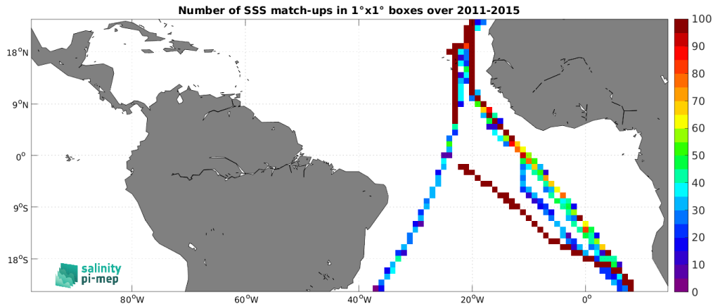
Figure 4: Number of SSS match-ups between TSG (Polarstern) SSS and the Aquarius SSS L3 OR v5 - Monthly (NASA-GSFC) SSS product for the Tropical Atlantic Ocean Pi-MEP region over 1^\circ \times 1^\circ boxes and for the full satellite product period.
