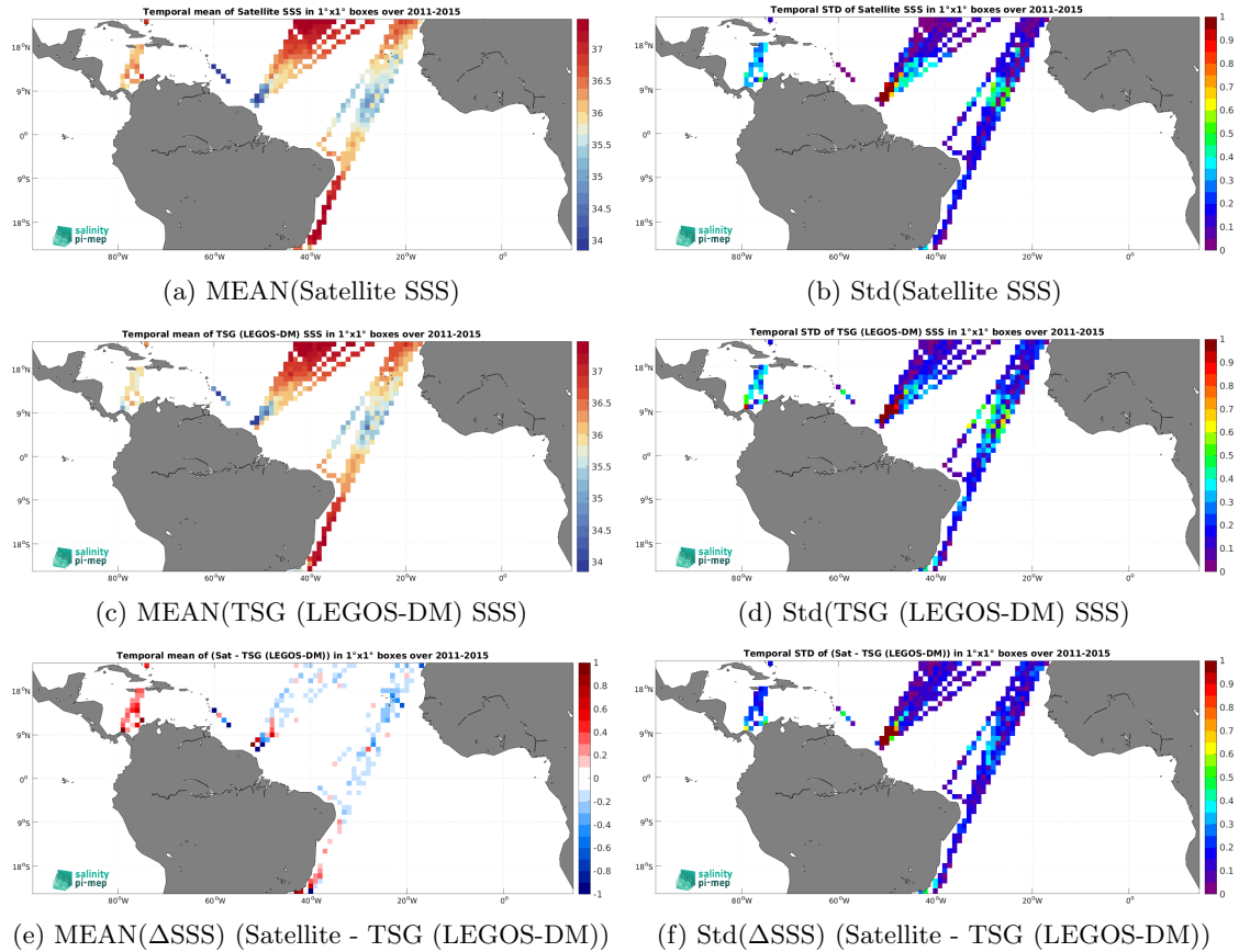
Figure 7: Temporal mean (left) and Std (right) of SSS from Aquarius SSS L3 OR v5 - Monthly (NASA-GSFC) (top), TSG (LEGOS-DM) (middle), and of \Delta\text{SSS} (Satellite - TSG (LEGOS-DM)). Only match-up pairs are used to generate these maps.
