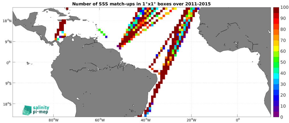
Figure 5: Number of SSS match-ups between TSG (LEGOS-DM) SSS and the Aquarius SSS L3 OR v5 - Monthly (NASA-GSFC) SSS product for the Tropical Atlantic Ocean Pi-MEP region over 1^\circ \times 1^\circ boxes and for the full satellite product period.
