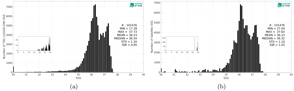
Figure 3: Histograms of SSS from TSG (LEGOS-DM) (a) and Aquarius SSS L3 OR v5 - Monthly (NASA-GSFC) (b) considering all match-up pairs per bins of 0.1 over the Tropical Atlantic Ocean Pi-MEP region and for the full satellite product period.
