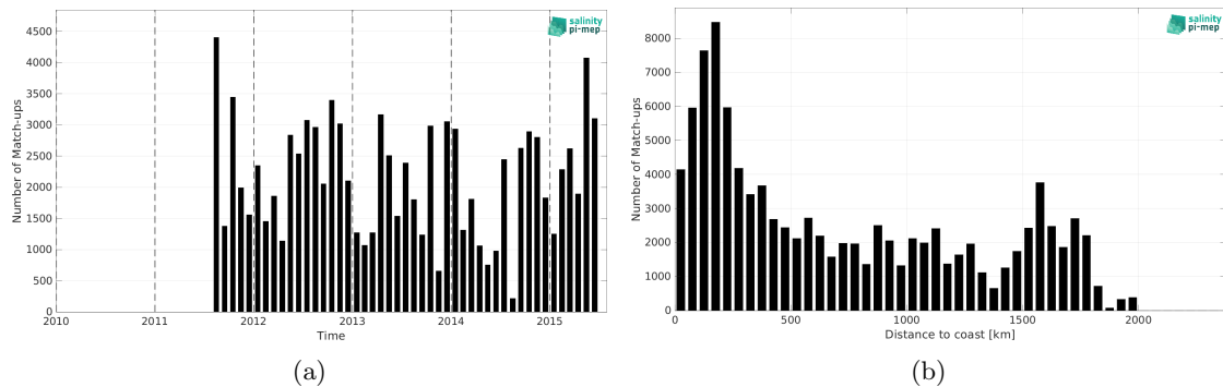
Figure 2: Number of match-ups between TSG (LEGOS-DM) and Aquarius SSS L3 OR v5 - Monthly (NASA-GSFC) SSS as a function of time (a) and as function of the distance to coast (b) over the Tropical Atlantic Ocean Pi-MEP region and for the full satellite product period.
