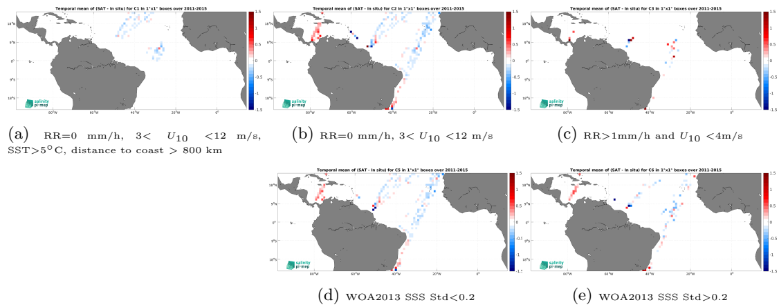
Figure 14: Temporal mean gridded over spatial boxes of size 1^\circ \times 1^\circ of \Delta SSS (Aquarius SSS L3 OR v5 - Monthly (NASA-GSFC) - TSG (LEGOS-DM)) for 5 different subdatasets corresponding to:RR=0 mm/h, 3 < U_{10} < 12 m/s, SST >5^\circ\text{C} , distance to coast > 800 km (a), RR=0 mm/h, 3 < U_{10} < 12 m/s (b), RR >1 mm/h and U_{10} < 4 m/s (c), WOA2013 SSS Std <0.2 (d), WOA2013 SSS Std >0.2 (e).
