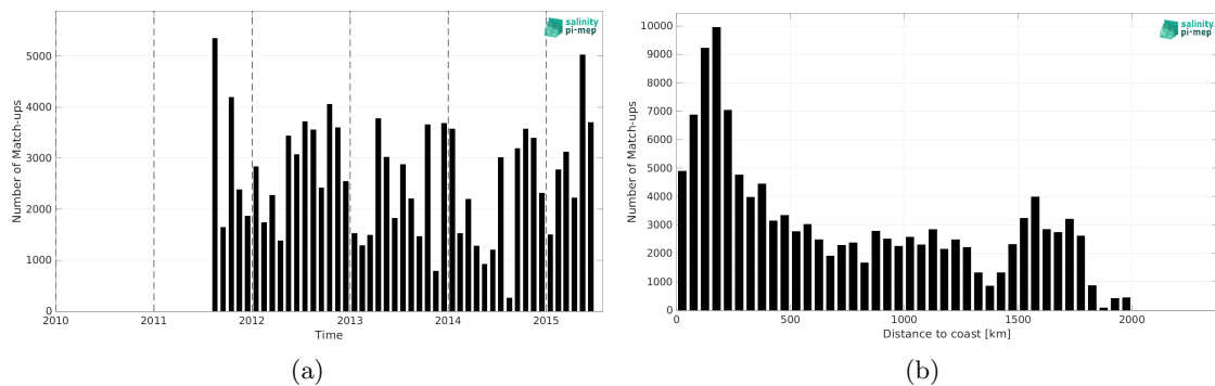
Figure 1: Number of match-ups between TSG (LEGOS-DM) and Aquarius SSS L3 OR v5 - Monthly (NASA-GSFC) SSS as a function of time (a) and as function of the distance to coast (b) over the Tropical Atlantic Ocean Pi-MEP region and for the full satellite product period.
