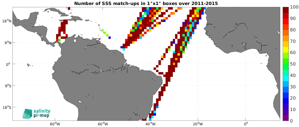
Figure 4: Number of SSS match-ups between TSG (LEGOS-DM) SSS and the Aquarius SSS L3 OR v5 - Monthly (NASA-GSFC) SSS product for the Tropical Atlantic Ocean Pi-MEP region over 1^\circ \times 1^\circ boxes and for the full satellite product period.
