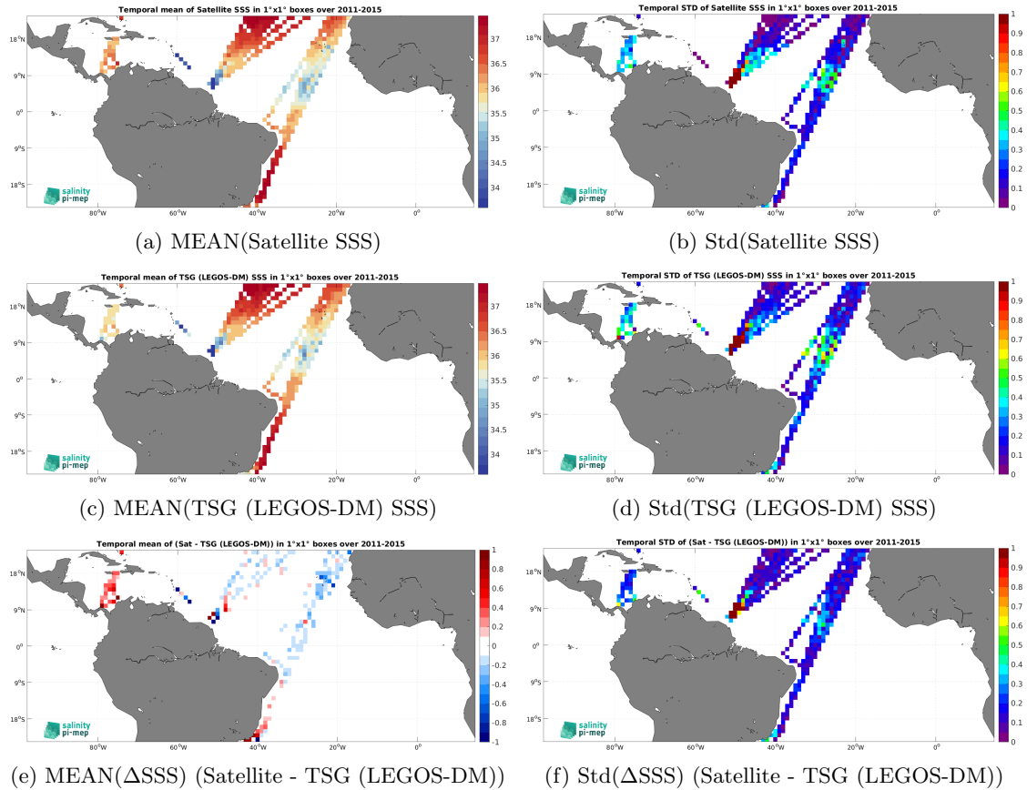
Figure 6: Temporal mean (left) and Std (right) of SSS from Aquarius SSS L3 OR v5 - Monthly (NASA-GSFC) (top), TSG (LEGOS-DM) (middle), and of \Delta\text{SSS} (Satellite - TSG (LEGOS-DM)). Only match-up pairs are used to generate these maps.
