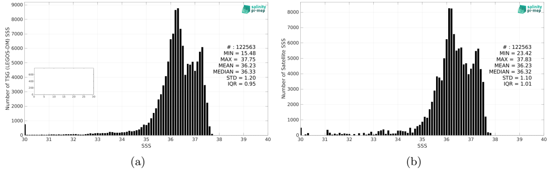
Figure 2: Histograms of SSS from TSG (LEGOS-DM) (a) and Aquarius SSS L3 OR v5 - Monthly (NASA-GSFC) (b) considering all match-up pairs per bins of 0.1 over the Tropical Atlantic Ocean Pi-MEP region and for the full satellite product period.
