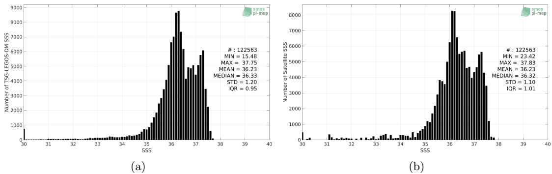
Figure 2: Histograms of SSS from TSG-LEGOS-DM (a) and Aquarius-L3-OR-V5-MONTHLY-1DEG (b) considering all match-up pairs per bins of 0.1 over the Tropical Atlantic Ocean Pi-MEP region and for the full satellite product period.
