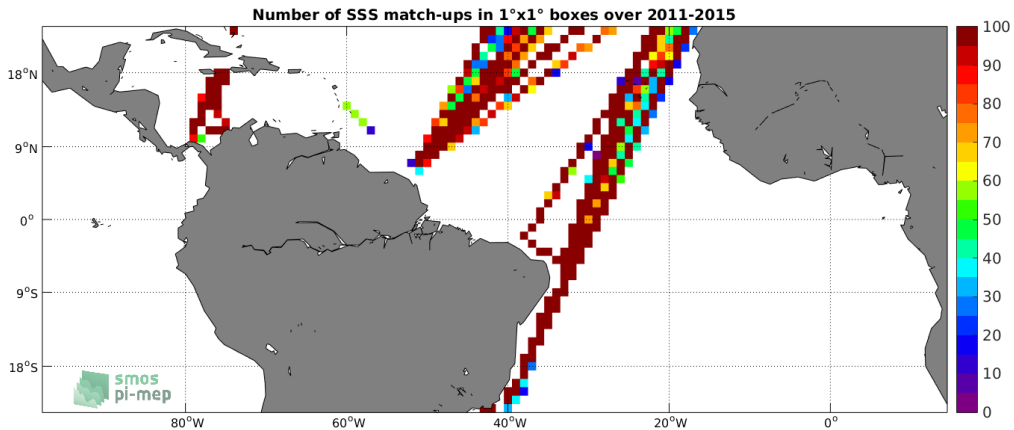
Figure 4: Number of SSS match-ups between TSG-LEGOS-DM SSS and the Aquarius-L3-OR-V5-MONTHLY-1DEG SSS product for the Tropical Atlantic Ocean Pi-MEP region over 1^\circ \times 1^\circ boxes and for the full satellite product period.
