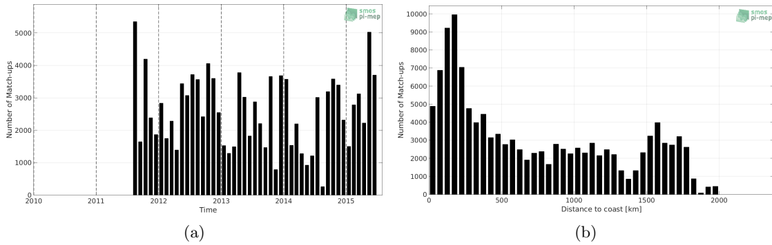
Figure 1: Number of match-ups between TSG-LEGOS-DM and Aquarius-L3-OR-V5-MONTHLY-1DEG SSS as a function of time (a) and as function of the distance to coast (b) over the Tropical Atlantic Ocean Pi-MEP region and for the full satellite product period.
