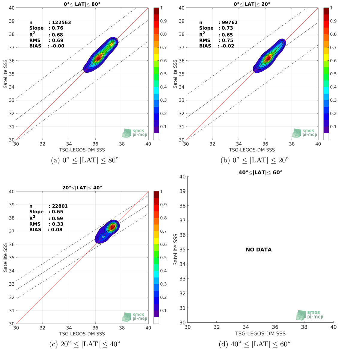
Figure 9: Contour maps of the concentration of Aquarius-L3-OR-V5-MONTHLY-1DEG SSS (y-axis) versus TSG-LEGOS-DM SSS (x-axis) at match-up pairs for different latitude bands. For each plot, the red line shows x=y . The black thin and dashed lines indicate a linear fit through the data cloud and the \pm 95\% confidence levels, respectively. The number match-up pairs n , the slope and R^2 coefficient of the linear fit, the root mean square (RMS) and the mean bias between satellite and in situ data are indicated for each latitude band in each plots.
