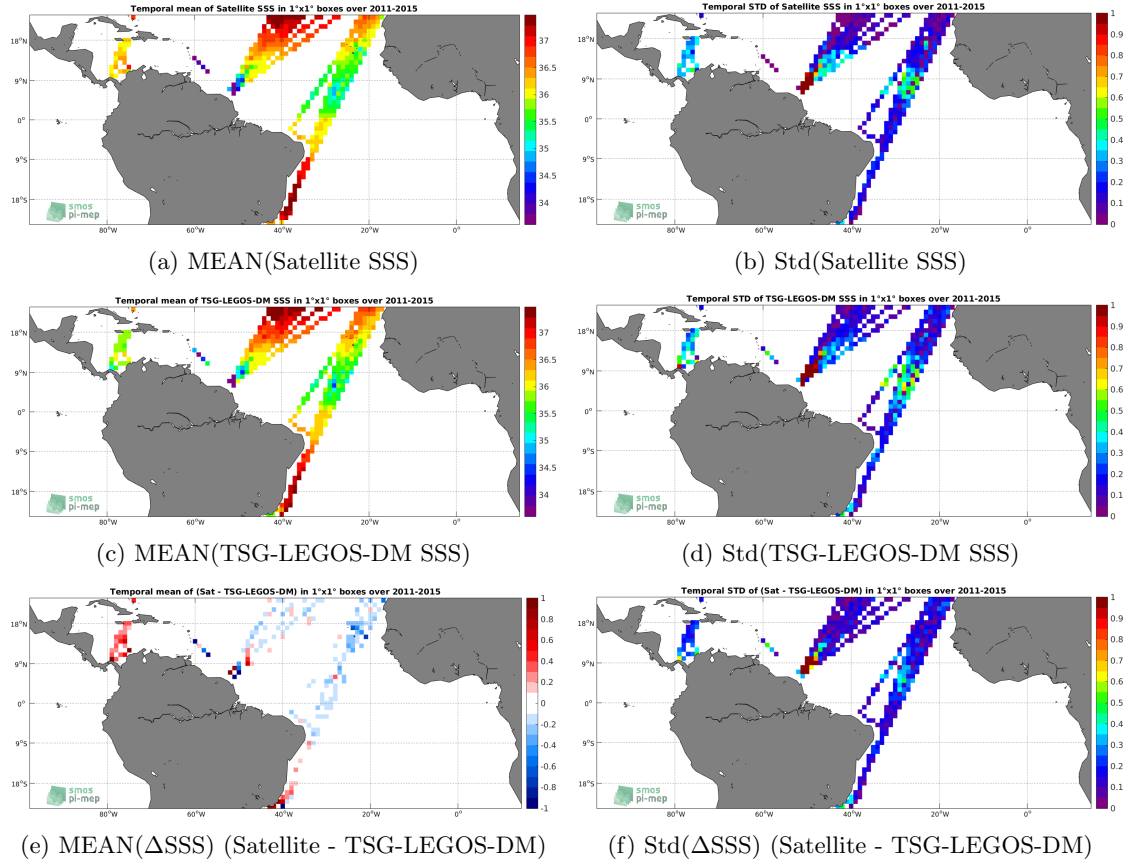
Figure 6: Temporal mean (left) and Std (right) of SSS from Aquarius-L3-OR-V5-MONTHLY-1DEG (top), TSG-LEGOS-DM (middle), and of \Delta SSS (Satellite - TSG-LEGOS-DM). Only match-up pairs are used to generate these maps.
