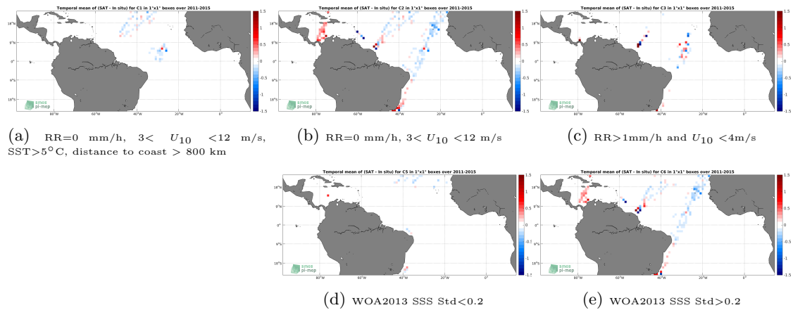
Figure 12: Temporal mean gridded over spatial boxes of size 1^\circ \times 1^\circ of \Delta SSS (Aquarius-L3-OR-V5-MONTHLY-1DEG - TSG-LEGOS-DM) for 5 different subdatasets corresponding to:RR=0 mm/h, 3 < U_{10} < 12 m/s, SST >5^\circ\text{C} , distance to coast > 800 km (a), RR=0 mm/h, 3 < U_{10} < 12 m/s (b), RR >1 mm/h and U_{10} < 4 m/s (c), WOA2013 SSS Std <0.2 (d), WOA2013 SSS Std >0.2 (e).
