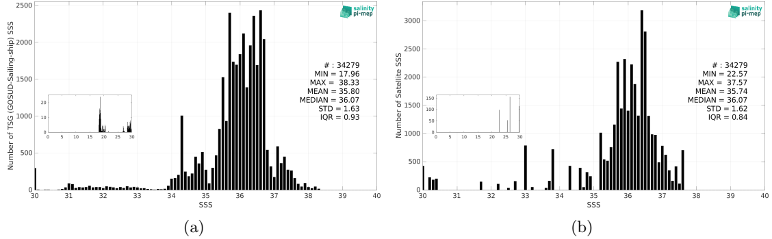
Figure 3: Histograms of SSS from TSG (GOSUD-Sailing-ship) (a) and Aquarius SSS L3 OR v5 - Monthly (NASA-GSFC) (b) considering all match-up pairs per bins of 0.1 over the Tropical Atlantic Ocean Pi-MEP region and for the full satellite product period.
