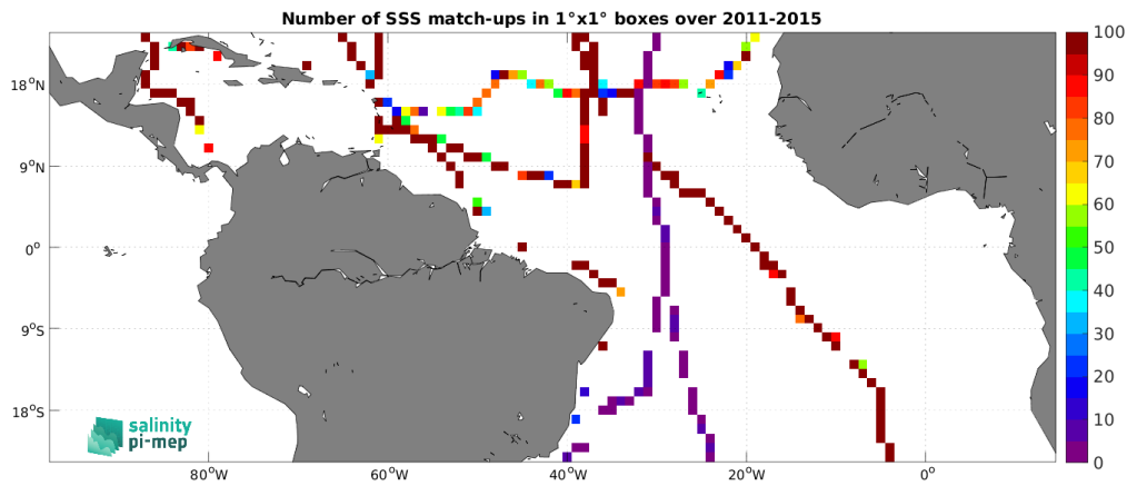
Figure 5: Number of SSS match-ups between TSG (GOSUD-Sailing-ship) SSS and the Aquarius SSS L3 OR v5 - Monthly (NASA-GSFC) SSS product for the Tropical Atlantic Ocean Pi-MEP region over 1^\circ \times 1^\circ boxes and for the full satellite product period.
