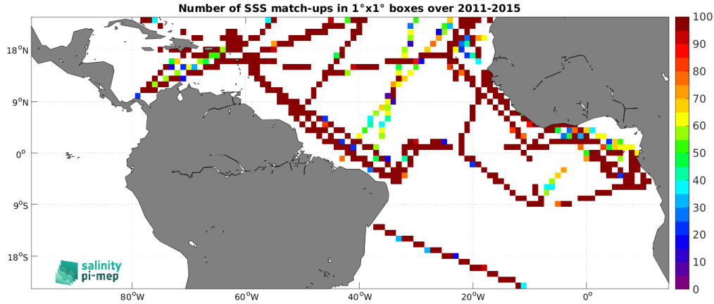
Figure 5: Number of SSS match-ups between TSG (GOSUD-Research-vessel) SSS and the Aquarius SSS L3 OR v5 - Monthly (NASA-GSFC) SSS product for the Tropical Atlantic Ocean Pi-MEP region over 1^\circ \times 1^\circ boxes and for the full satellite product period.
