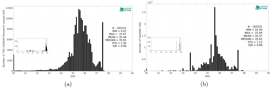
Figure 3: Histograms of SSS from TSG (GOSUD-Research-vessel) (a) and Aquarius SSS L3 OR v5 - Monthly (NASA-GSFC) (b) considering all match-up pairs per bins of 0.1 over the Tropical Atlantic Ocean Pi-MEP region and for the full satellite product period.
