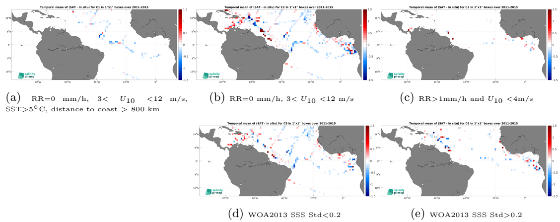
Figure 14: Temporal mean gridded over spatial boxes of size 1^\circ \times 1^\circ of \Delta\text{SSS} (Aquarius SSS L3 OR v5 - Monthly (NASA-GSFC) - TSG (GOSUD-Research-vessel)) for 5 different subdatasets corresponding to:RR=0 mm/h, 3 < U_{10} < 12 m/s, SST >5^\circ\text{C} , distance to coast > 800 km (a), RR=0 mm/h, 3 < U_{10} < 12 m/s (b), RR >1 mm/h and U_{10} < 4 m/s (c), WOA2013 SSS Std <0.2 (d), WOA2013 SSS Std >0.2 (e).
