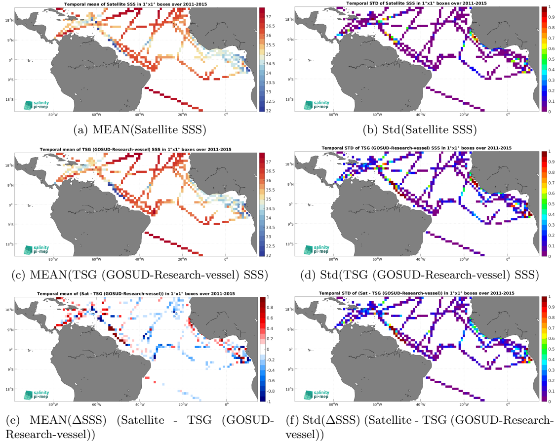
Figure 7: Temporal mean (left) and Std (right) of SSS from Aquarius SSS L3 OR v5 - Monthly (NASA-GSFC) (top), TSG (GOSUD-Research-vessel) (middle), and of \Delta\text{SSS} (Satellite - TSG (GOSUD-Research-vessel)). Only match-up pairs are used to generate these maps.
