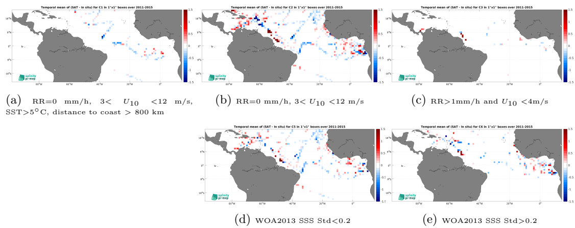
Figure 12: Temporal mean gridded over spatial boxes of size 1^\circ \times 1^\circ of \Delta SSS (Aquarius SSS L3 OR v5 - Monthly (NASA-GSFC) - TSG (GOSUD-Research-vessel)) for 5 different subdatasets corresponding to:RR=0 mm/h, 3 < U_{10} < 12 m/s, SST >5^\circ\text{C} , distance to coast > 800 km (a), RR=0 mm/h, 3 < U_{10} < 12 m/s (b), RR >1 mm/h and U_{10} < 4 m/s (c), WOA2013 SSS Std <0.2 (d), WOA2013 SSS Std >0.2 (e).
