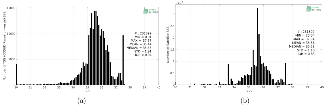
Figure 2: Histograms of SSS from TSG (GOSUD-Research-vessel) (a) and Aquarius SSS L3 OR v5 - Monthly (NASA-GSFC) (b) considering all match-up pairs per bins of 0.1 over the Tropical Atlantic Ocean Pi-MEP region and for the full satellite product period.
