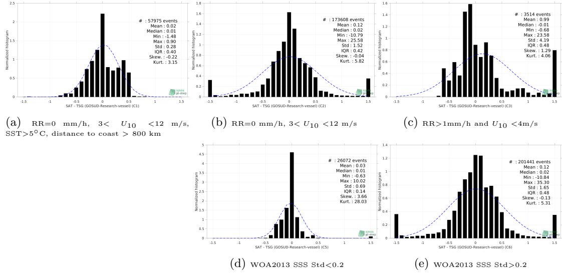
Figure 13: Normalized histogram of \Delta\text{SSS} (Aquarius SSS L3 OR v5 - Monthly (NASA-GSFC) - TSG (GOSUD-Research-vessel)) for 5 different subdatasets corresponding to: RR=0 mm/h, 3 < U_{10} < 12 m/s, SST>5°C, distance to coast > 800 km (a), RR=0 mm/h, 3 < U_{10} < 12 m/s (b), RR>1mm/h and U_{10} < 4 m/s (c), WOA2013 SSS Std<0.2 (d), WOA2013 SSS Std>0.2 (e).
