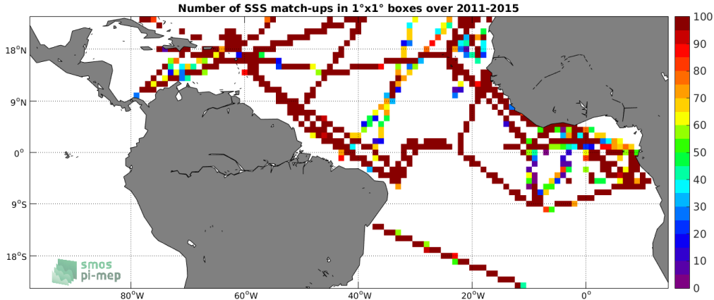
Figure 4: Number of SSS match-ups between TSG-GOSUD-Research-vessel SSS and the Aquarius-L3-OR-V5-MONTHLY-1DEG SSS product for the Tropical Atlantic Ocean Pi-MEP region over 1^\circ \times 1^\circ boxes and for the full satellite product period.
