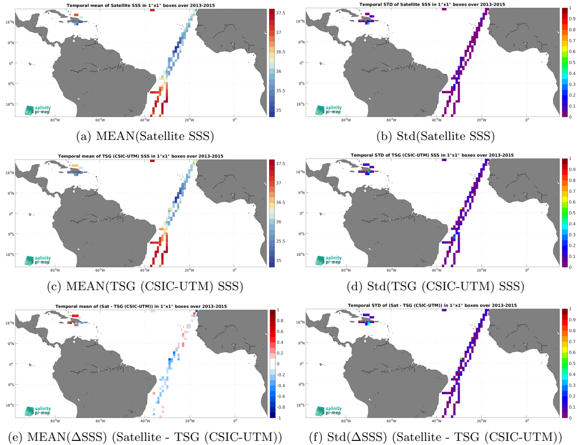
Figure 6: Temporal mean (left) and Std (right) of SSS from Aquarius SSS L3 OR v5 - Monthly (NASA-GSFC) (top), TSG (CSIC-UTM) ( in situ ) dataset (middle), and of \Delta\text{SSS}(\text{Satellite} - \text{TSG}(\text{CSIC-UTM})) . Only match-up pairs are used to generate these maps.
