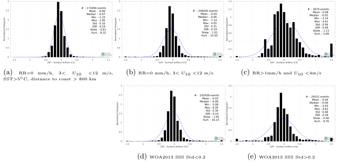
Figure 12: Normalized histogram of \Delta SSS (Aquarius SSS L3 OR v5 - Monthly (NASA-GSFC) - Surface drifters) for 5 different subdatasets corresponding to: RR=0 mm/h, 3 < U_{10} < 12 m/s, SST >5^{\circ} C, distance to coast > 800 km (a), RR=0 mm/h, 3 < U_{10} < 12 m/s (b), RR >1 mm/h and U_{10} < 4 m/s (c), WOA2013 SSS Std <0.2 (d), WOA2013 SSS Std >0.2 (e).
