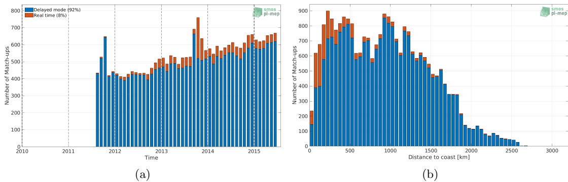
Figure 1: Number of match-ups between Argo and Aquarius SSS L3 OR v5 - Monthly (NASA-GSFC) SSS as a function of time (a) and as function of the distance to coast (b) over the Tropical Atlantic Ocean Pi-MEP region and for the full satellite product period.
