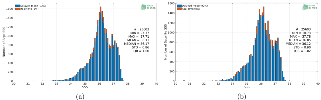
Figure 2: Histograms of SSS from Argo (a) and Aquarius SSS L3 OR v5 - Monthly (NASA-GSFC) (b) considering all match-up pairs per bins of 0.1 over the Tropical Atlantic Ocean Pi-MEP region and for the full satellite product period.
