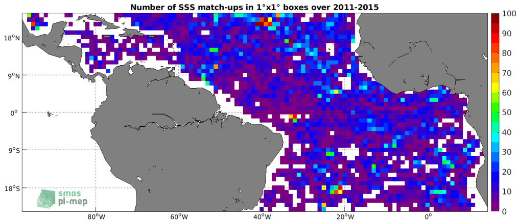
Figure 4: Number of SSS match-ups between Argo SSS and the Aquarius SSS L3 OR v5 - Monthly (NASA-GSFC) SSS product for the Tropical Atlantic Ocean Pi-MEP region over 1^\circ \times 1^\circ boxes and for the full satellite product period.
