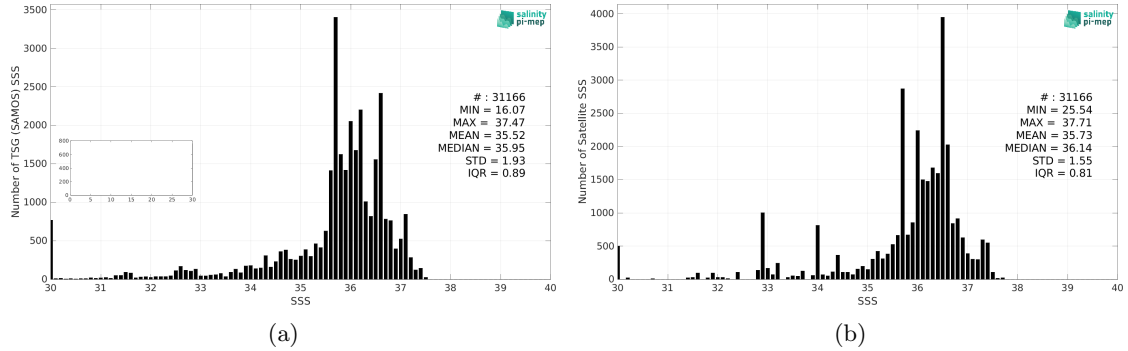
Figure 2: Histograms of SSS from TSG (SAMOS) (a) and Aquarius SSS L3 OR v5 - Monthly - Rain mask (NASA-GSFC) (b) considering all match-up pairs per bins of 0.1 over the Tropical Atlantic Ocean Pi-MEP region and for the full satellite product period.
