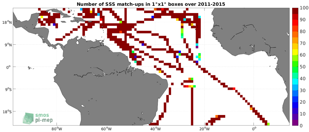
Figure 4: Number of SSS match-ups between TSG (SAMOS) SSS and the Aquarius SSS L3 OR v5 - Monthly - Rain mask (NASA-GSFC) SSS product for the Tropical Atlantic Ocean Pi-MEP region over 1^\circ \times 1^\circ boxes and for the full satellite product period.
