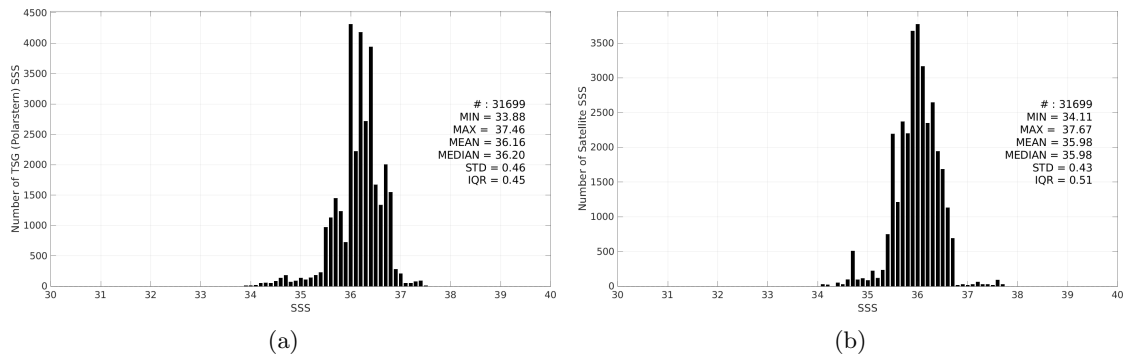
Figure 3: Histograms of SSS from TSG (Polarstern) (a) and Aquarius SSS L3 OR v5 - Monthly - Rain mask (NASA-GSFC) (b) considering all match-up pairs per bins of 0.1 over the Tropical Atlantic Ocean Pi-MEP region and for the full satellite product period.
