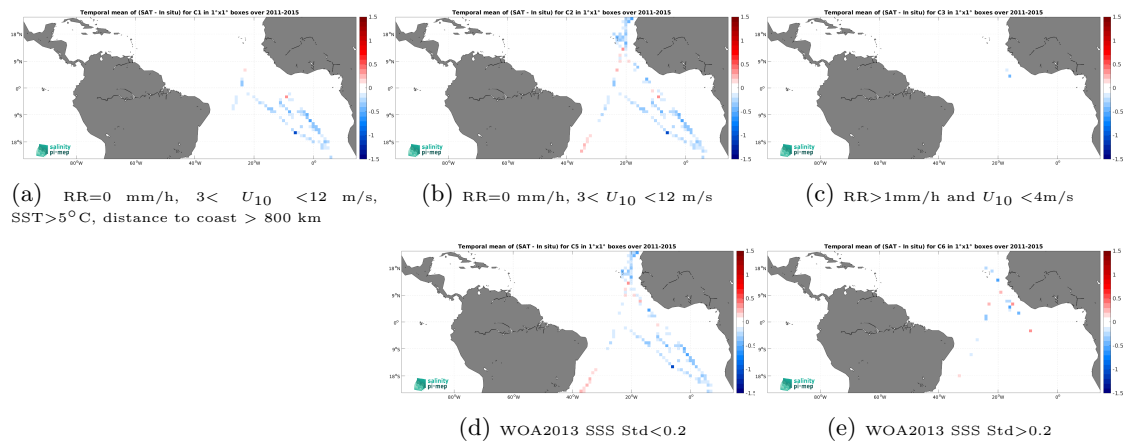
Figure 14: Temporal mean gridded over spatial boxes of size 1^\circ \times 1^\circ of \Delta SSS (Aquarius SSS L3 OR v5 - Monthly - Rain mask (NASA-GSFC) - TSG (Polarstern)) for 5 different subdatasets corresponding to:RR=0 mm/h, 3 < U_{10} < 12 m/s, SST >5^\circ\text{C} , distance to coast > 800 km (a), RR=0 mm/h, 3 < U_{10} < 12 m/s (b), RR >1 mm/h and U_{10} < 4 m/s (c), WOA2013 SSS Std <0.2 (d), WOA2013 SSS Std >0.2 (e).
