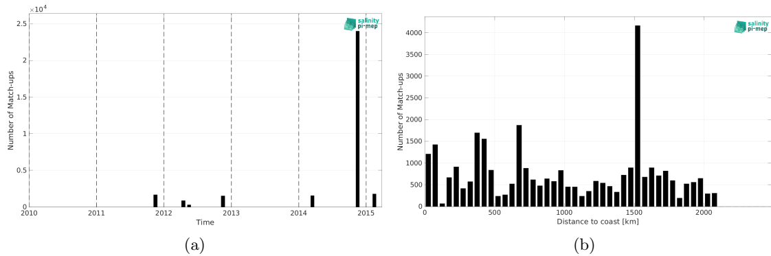
Figure 2: Number of match-ups between TSG (Polarstern) and Aquarius SSS L3 OR v5 - Monthly - Rain mask (NASA-GSFC) SSS as a function of time (a) and as function of the distance to coast (b) over the Tropical Atlantic Ocean Pi-MEP region and for the full satellite product period.
