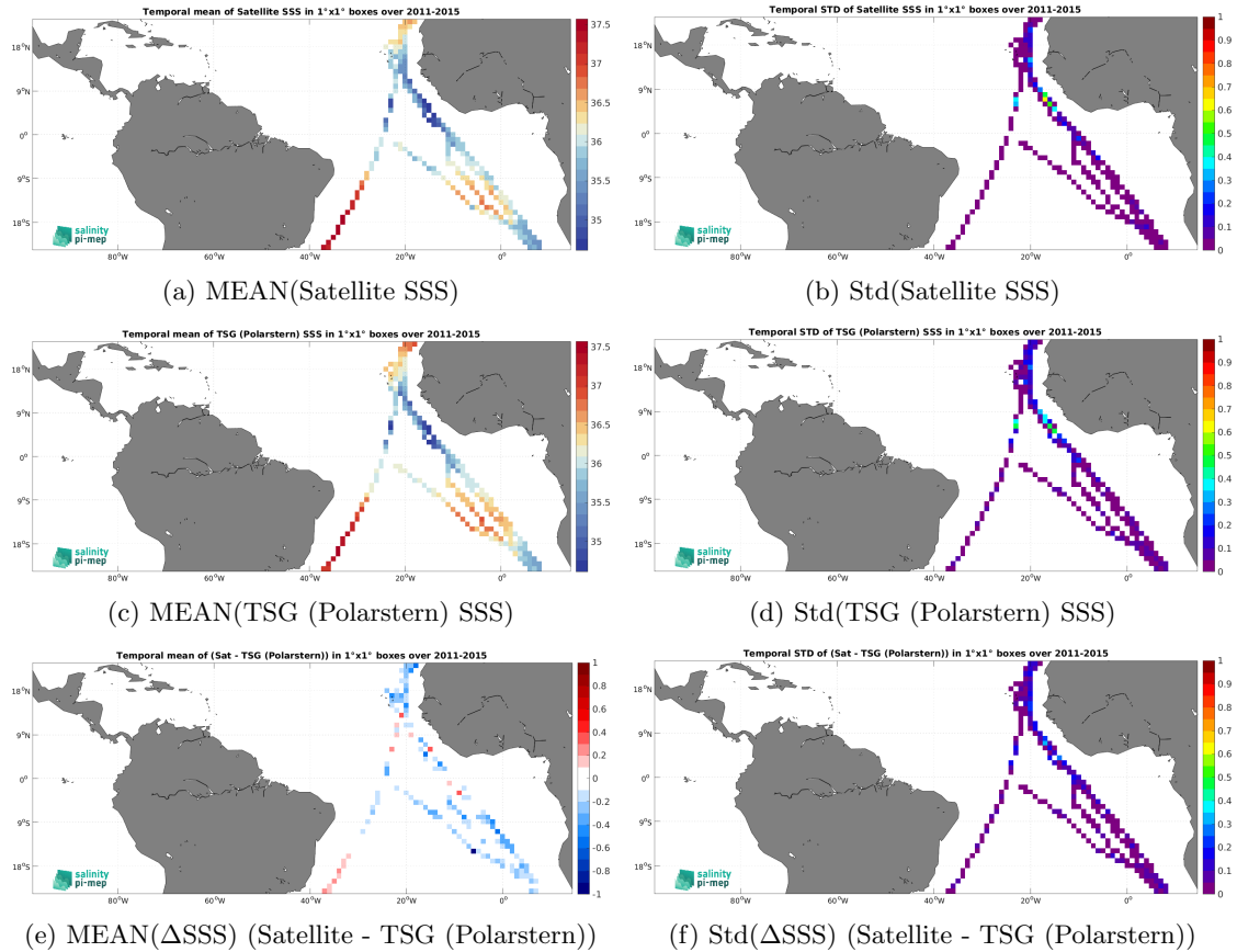
Figure 7: Temporal mean (left) and Std (right) of SSS from Aquarius SSS L3 OR v5 - Monthly - Rain mask (NASA-GSFC) (top), TSG (Polarstern) (middle), and of \Delta SSS (Satellite - TSG (Polarstern)). Only match-up pairs are used to generate these maps.
