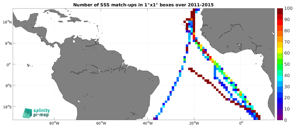
Figure 5: Number of SSS match-ups between TSG (Polarstern) SSS and the Aquarius SSS L3 OR v5 - Monthly - Rain mask (NASA-GSFC) SSS product for the Tropical Atlantic Ocean Pi-MEP region over 1^\circ \times 1^\circ boxes and for the full satellite product period.
