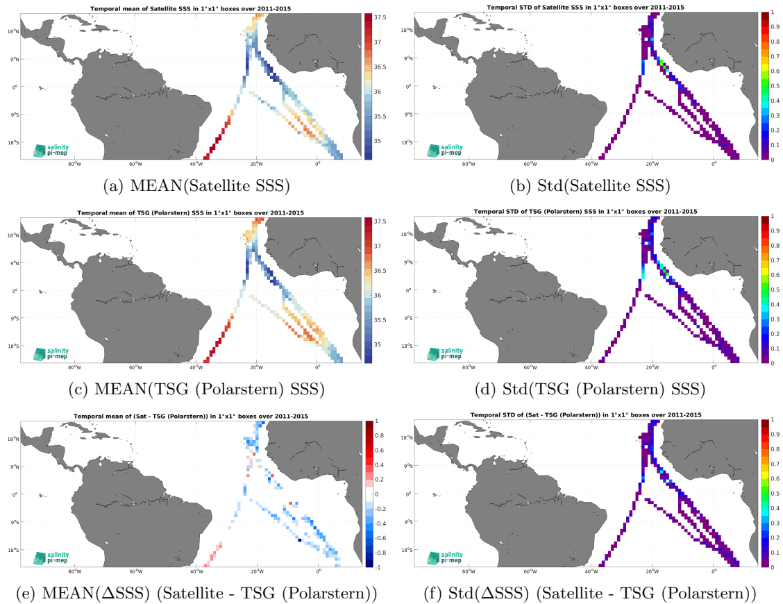
Figure 6: Temporal mean (left) and Std (right) of SSS from Aquarius SSS L3 OR v5 - Monthly - Rain mask (NASA-GSFC) (top), TSG (Polarstern) (middle), and of \Delta SSS (Satellite - TSG (Polarstern)). Only match-up pairs are used to generate these maps.
