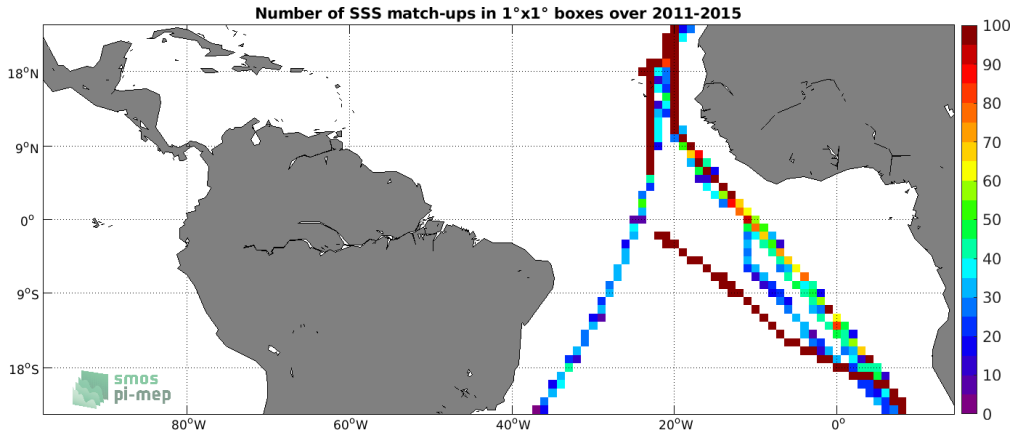
Figure 4: Number of SSS match-ups between TSG (Polarstern) SSS and the Aquarius SSS L3 OR v5 - Monthly - Rain mask (NASA-GSFC) SSS product for the Tropical Atlantic Ocean Pi-MEP region over 1^\circ \times 1^\circ boxes and for the full satellite product period.
