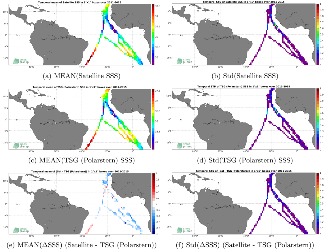
Figure 6: Temporal mean (left) and Std (right) of SSS from Aquarius SSS L3 OR v5 - Monthly - Rain mask (NASA-GSFC) (top), TSG (Polarstern) (middle), and of \Delta\text{SSS} (Satellite - TSG (Polarstern)). Only match-up pairs are used to generate these maps.
