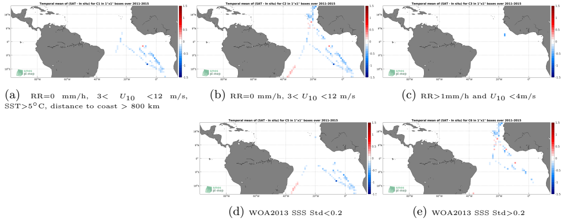
Figure 12: Temporal mean gridded over spatial boxes of size 1^{\circ}\times 1^{\circ} of \Delta\text{SSS} (Aquarius SSS L3 OR v5 - Monthly - Rain mask (NASA-GSFC) - TSG (Polarstern)) for 5 different subdatasets corresponding to:RR=0 mm/h, 3 < U_{10} < 12 m/s, SST >5^{\circ}\text{C} , distance to coast > 800 km (a), RR=0 mm/h, 3 < U_{10} < 12 m/s (b), RR >1 mm/h and U_{10} < 4 m/s (c), WOA2013 SSS Std <0.2 (d), WOA2013 SSS Std >0.2 (e).
