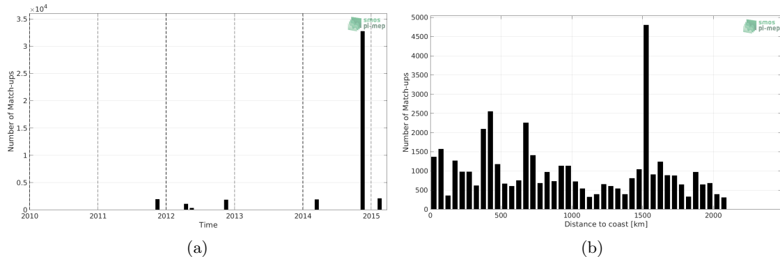
Figure 1: Number of match-ups between TSG (Polarstern) and Aquarius SSS L3 OR v5 - Monthly - Rain mask (NASA-GSFC) SSS as a function of time (a) and as function of the distance to coast (b) over the Tropical Atlantic Ocean Pi-MEP region and for the full satellite product period.
