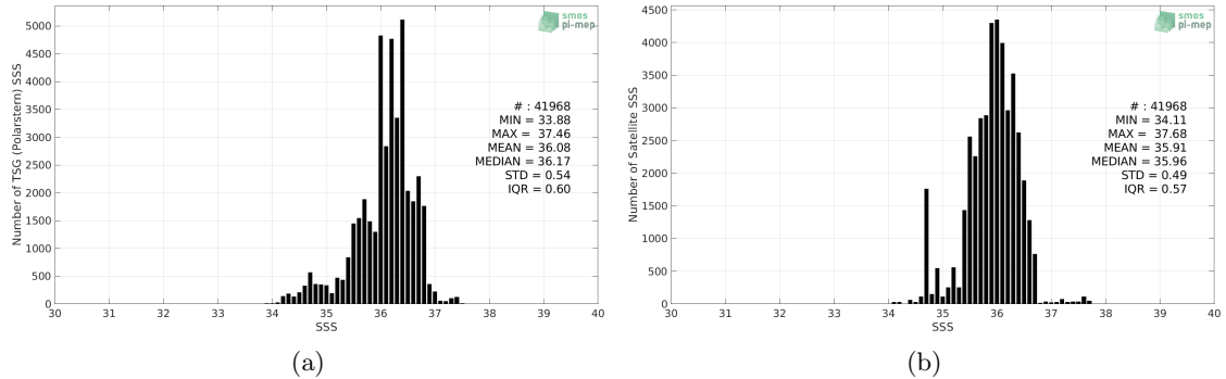
Figure 2: Histograms of SSS from TSG (Polarstern) (a) and Aquarius SSS L3 OR v5 - Monthly - Rain mask (NASA-GSFC) (b) considering all match-up pairs per bins of 0.1 over the Tropical Atlantic Ocean Pi-MEP region and for the full satellite product period.
