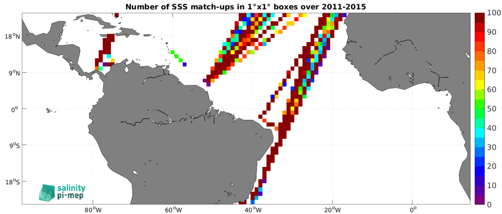
Figure 5: Number of SSS match-ups between TSG (LEGOS-DM) SSS and the Aquarius SSS L3 OR v5 - Monthly - Rain mask (NASA-GSFC) SSS product for the Tropical Atlantic Ocean Pi-MEP region over 1^\circ \times 1^\circ boxes and for the full satellite product period.
