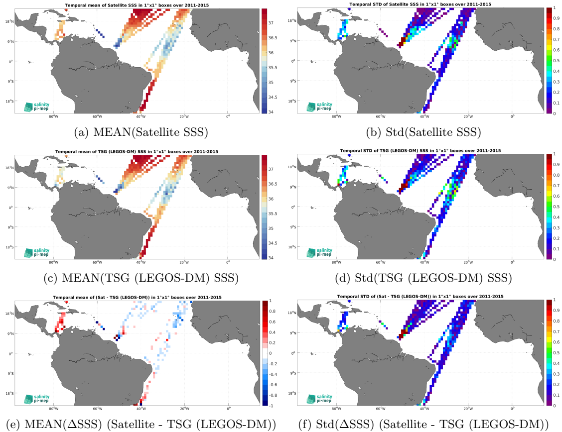
Figure 7: Temporal mean (left) and Std (right) of SSS from Aquarius SSS L3 OR v5 - Monthly - Rain mask (NASA-GSFC) (top), TSG (LEGOS-DM) (middle), and of \Delta\text{SSS} (Satellite - TSG (LEGOS-DM)). Only match-up pairs are used to generate these maps.
