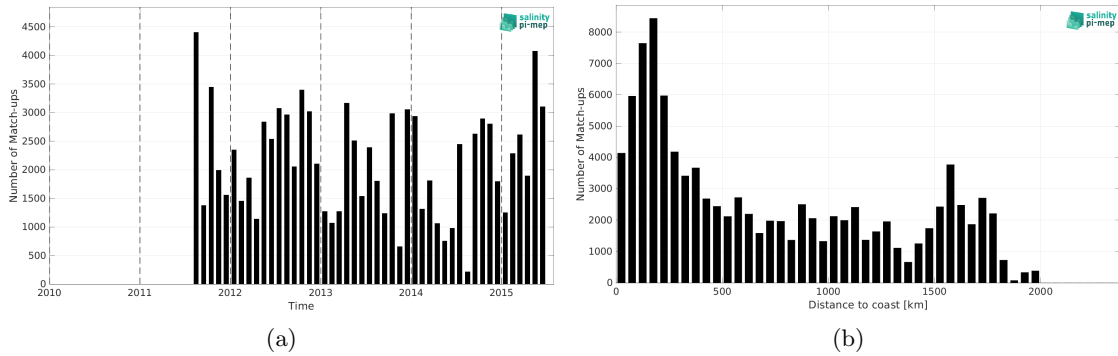
Figure 2: Number of match-ups between TSG (LEGOS-DM) and Aquarius SSS L3 OR v5 - Monthly - Rain mask (NASA-GSFC) SSS as a function of time (a) and as function of the distance to coast (b) over the Tropical Atlantic Ocean Pi-MEP region and for the full satellite product period.
