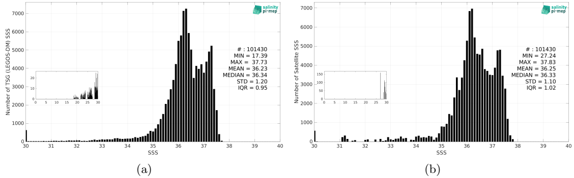
Figure 3: Histograms of SSS from TSG (LEGOS-DM) (a) and Aquarius SSS L3 OR v5 - Monthly - Rain mask (NASA-GSFC) (b) considering all match-up pairs per bins of 0.1 over the Tropical Atlantic Ocean Pi-MEP region and for the full satellite product period.
