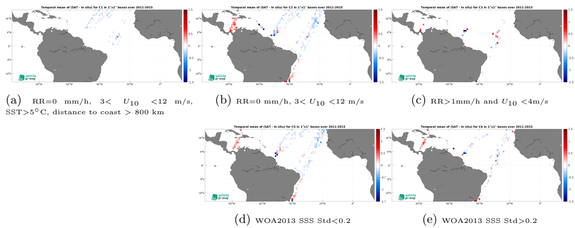
Figure 14: Temporal mean gridded over spatial boxes of size 1^\circ \times 1^\circ of \Delta\text{SSS} (Aquarius SSS L3 OR v5 - Monthly - Rain mask (NASA-GSFC) - TSG (LEGOS-DM)) for 5 different subdatasets corresponding to:RR=0 mm/h, 3 < U_{10} < 12 m/s, SST>5°C, distance to coast > 800 km (a), RR=0 mm/h, 3 < U_{10} < 12 m/s (b), RR>1mm/h and U_{10} < 4 m/s (c), WOA2013 SSS Std<0.2 (d), WOA2013 SSS Std>0.2 (e).
