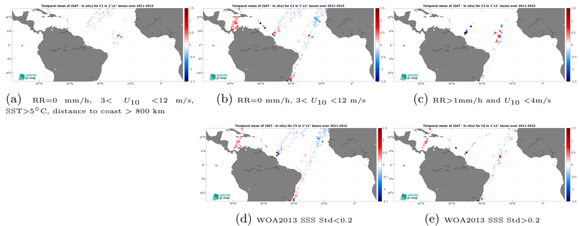
Figure 12: Temporal mean gridded over spatial boxes of size 1^\circ \times 1^\circ of \Delta\text{SSS} (Aquarius SSS L3 OR v5 - Monthly - Rain mask (NASA-GSFC) - TSG (LEGOS-DM)) for 5 different subdatasets corresponding to:RR=0 mm/h, 3 < U_{10} < 12 m/s, SST >5^\circ\text{C} , distance to coast > 800 km (a), RR=0 mm/h, 3 < U_{10} < 12 m/s (b), RR >1 mm/h and U_{10} < 4 m/s (c), WOA2013 SSS Std <0.2 (d), WOA2013 SSS Std >0.2 (e).
