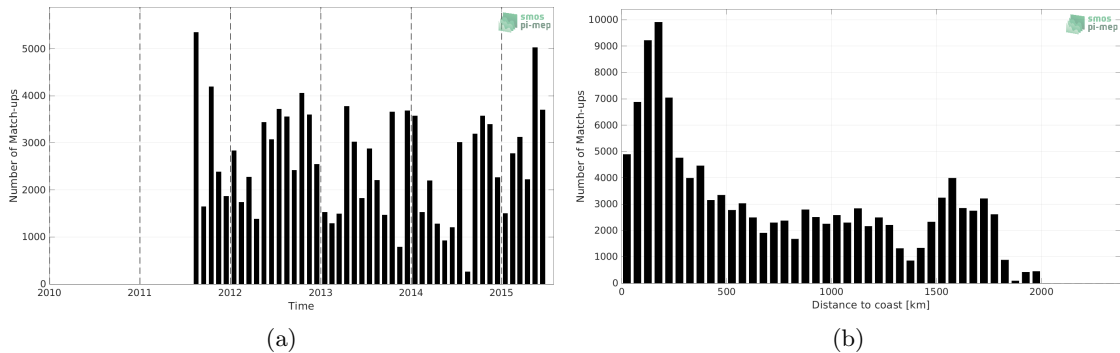
Figure 1: Number of match-ups between TSG (LEGOS-DM) and Aquarius SSS L3 OR v5 - Monthly - Rain mask (NASA-GSFC) SSS as a function of time (a) and as function of the distance to coast (b) over the Tropical Atlantic Ocean Pi-MEP region and for the full satellite product period.
