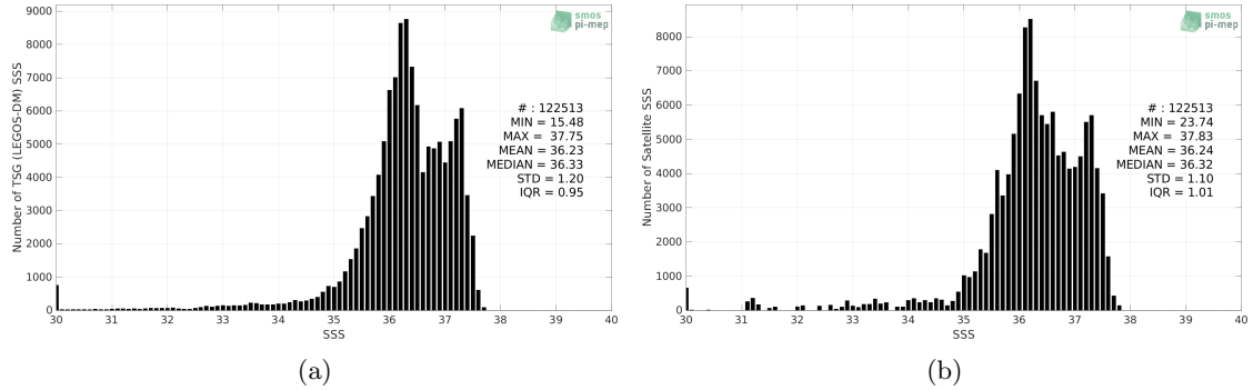
Figure 2: Histograms of SSS from TSG (LEGOS-DM) (a) and Aquarius SSS L3 OR v5 - Monthly - Rain mask (NASA-GSFC) (b) considering all match-up pairs per bins of 0.1 over the Tropical Atlantic Ocean Pi-MEP region and for the full satellite product period.
