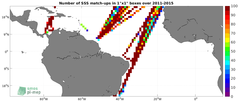
Figure 4: Number of SSS match-ups between TSG (LEGOS-DM) SSS and the Aquarius SSS L3 OR v5 - Monthly - Rain mask (NASA-GSFC) SSS product for the Tropical Atlantic Ocean Pi-MEP region over 1^\circ \times 1^\circ boxes and for the full satellite product period.
