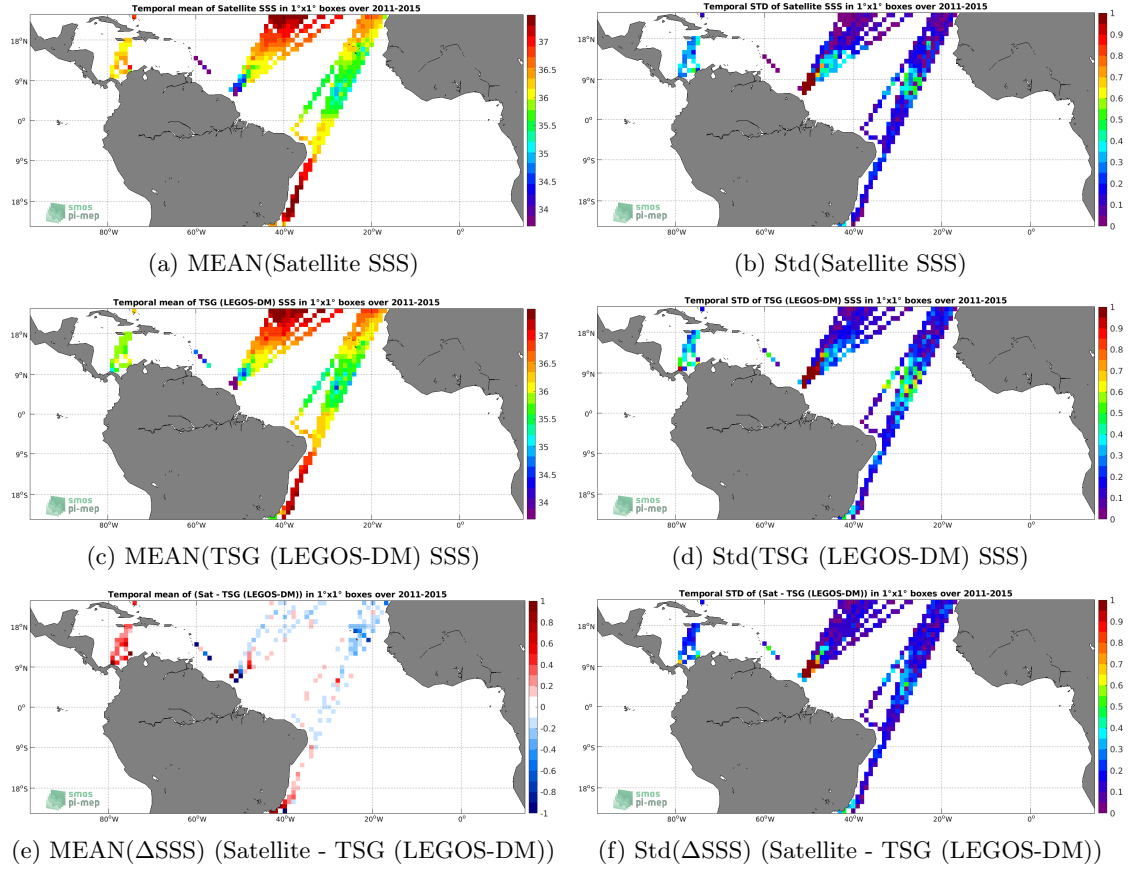
Figure 6: Temporal mean (left) and Std (right) of SSS from Aquarius SSS L3 OR v5 - Monthly - Rain mask (NASA-GSFC) (top), TSG (LEGOS-DM) (middle), and of \Delta SSS (Satellite - TSG (LEGOS-DM)). Only match-up pairs are used to generate these maps.
