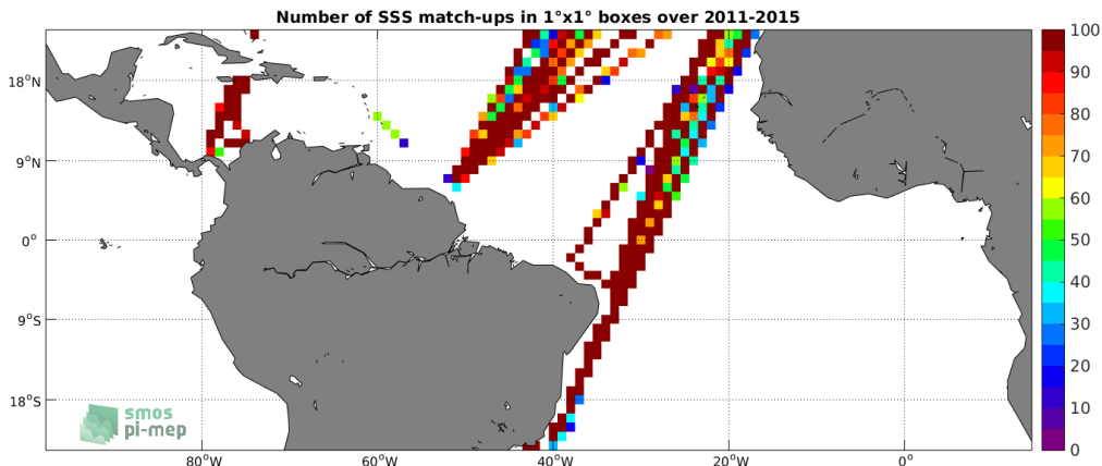
Figure 4: Number of SSS match-ups between TSG-LEGOS-DM SSS and the Aquarius-L3-OR-V5-MONTHLY-RAIN-MASK-1DEG SSS product for the Tropical Atlantic Ocean Pi-MEP region over 1^\circ \times 1^\circ boxes and for the full satellite product period.
