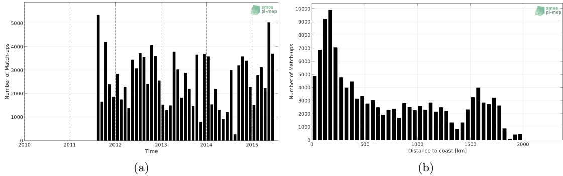
Figure 1: Number of match-ups between TSG-LEGOS-DM and Aquarius-L3-OR-V5-MONTHLY-RAIN-MASK-1DEG SSS as a function of time (a) and as function of the distance to coast (b) over the Tropical Atlantic Ocean Pi-MEP region and for the full satellite product period.
