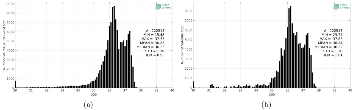
Figure 2: Histograms of SSS from TSG-LEGOS-DM (a) and Aquarius-L3-OR-V5-MONTHLY-RAIN-MASK-1DEG (b) considering all match-up pairs per bins of 0.1 over the Tropical Atlantic Ocean Pi-MEP region and for the full satellite product period.
