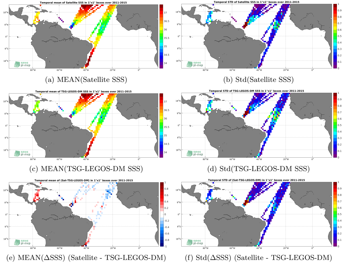
Figure 6: Temporal mean (left) and Std (right) of SSS from Aquarius-L3-OR-V5-MONTHLY-RAIN-MASK-1DEG (top), TSG-LEGOS-DM (middle), and of \Delta SSS (Satellite - TSG-LEGOS-DM). Only match-up pairs are used to generate these maps.
